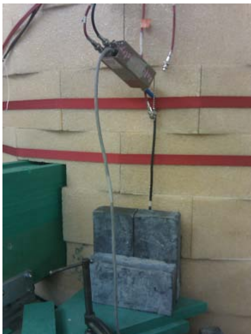
Figure 24. The outer shell of the NREP TMR is made from blocks of borated materials used to absorb neutrons and limit the radiation exposure to equipment located outside the TMR cylinder.
