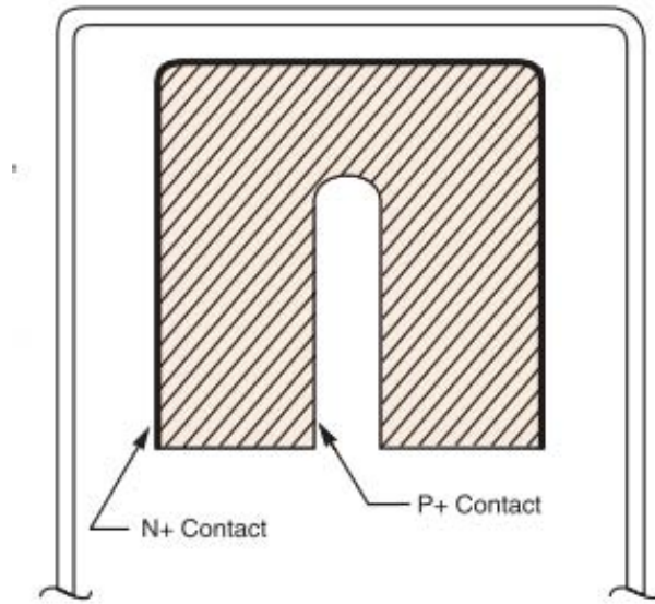
Figure 26. The schematic for a Standard Electrode Coaxial Germanium Detector displays an n -type contact and p -type contact sandwiching high-purity germanium (cross-hatched area) and surrounded by a cylindrical metal shell.
