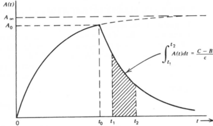
Figure 11. The activity of an irradiated foil is shown as a function of time, where A_{\infty} is the saturation activity, A_0 is the activity at the end of irradiation, t_0 is the end irradiation time, t_1 is the start count time, and t_2 is the end count time.
