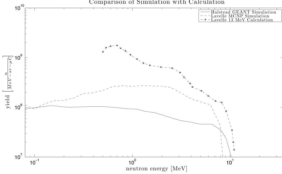
Figure 20. A comparison of the two simulation models with the calculations done in [25].
