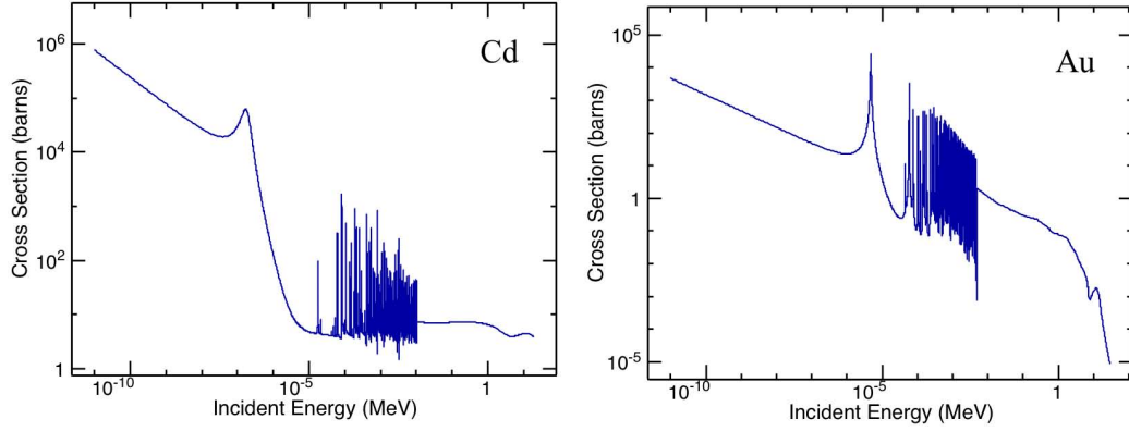
Figure 31. Left: The total cross section for ^{113}\text{Cd} for thermal through fast incident neutrons shows the cadmium cutoff, around 0.5 \text{ eV} [1]. Right: The cross section for ^{197}\text{Au} for the (n,\gamma) reaction [1].
