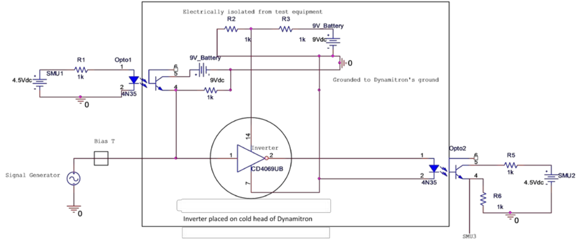
Figure 14. The schematic of test circuit A, where area II is electrically isolated from areas I and III. Voltage is swept from 0 to 4.5 V by an SMU in area I, while two SMUs measure and source in area III. Two 9 V are used in area II, one to source the inverter, while the other to source optoisolator 1.
