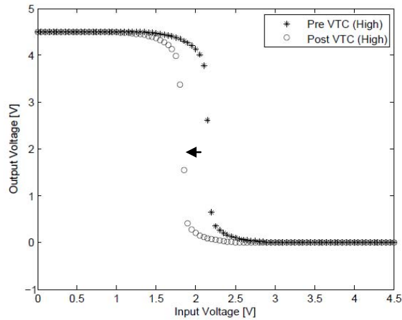
Figure 47. Pre-versus post-VTC of inverter being irradiated at 1 \mu A, a similar 0.3 V negative V_{th} was observed.
