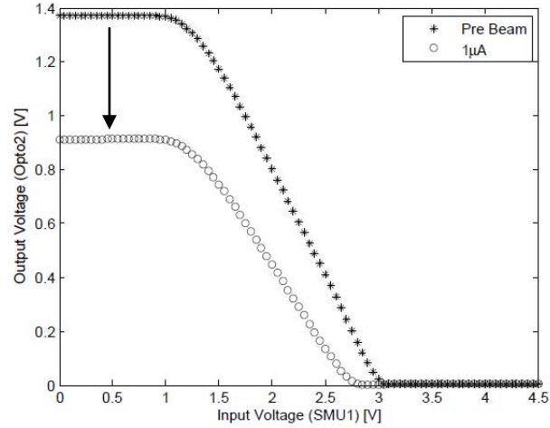
Figure 46. Inverter held high with a constant current applied at 1 \mu A. The same fluence of 7.06 \times 10^{14} \text{ [e}^-/\text{cm}^2] was obtained as in the previous two cases, but a flux of 1.7 \times 10^{12} \text{ [e}^-/\text{cm}^2 \text{ sec}] was achieved.
