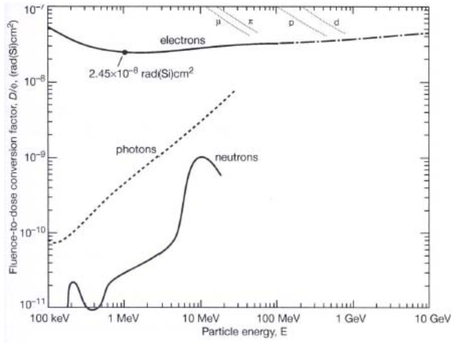
Figure 6. A fluence-to-dose conversion factor for a 1MeV electron [13].
