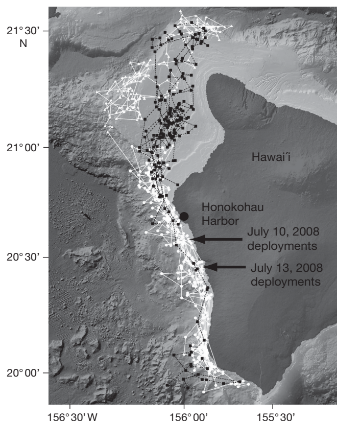
Fig. 3. Mesoplodon densirostris . Satellite-derived locations of Blainville's beaked whales tagged in 2008. HIMd007 (represented by the white circles and solid white line) is shown for the entire duration of signal contact, and because this whale traveled together with HIMd020 and HIMd036, its track is representative of movements by all 3 (see Fig. 4). HIMd025 (black squares and dashed black line) and HIMd148 (white triangles and solid white line, all north of 21° N) are shown for periods when they are separated from HIMd007 (see Fig. 4). HIMd025 and HIMd148 spent 41 and 31 % of their time, respectively, mirroring the movements of HIMd007. Lines joining consecutive points illustrate time series rather than actual travel routes
