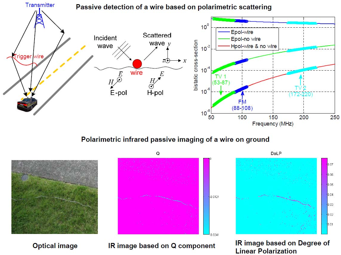
Fig 5: Passive detection methods for a long, thin wire in the presence of background scattering.
