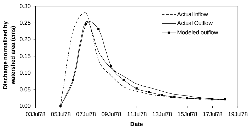
Figure 2-11. Results of Muskingum parameter calibration for runoff prediction at Dehraut.
