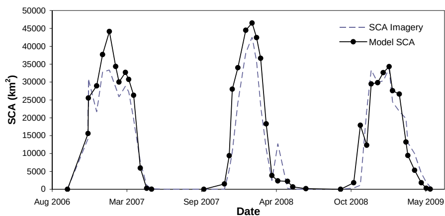
Figure 3-4. Time series comparison of modeled SCA and high-resolution SCA imagery.
