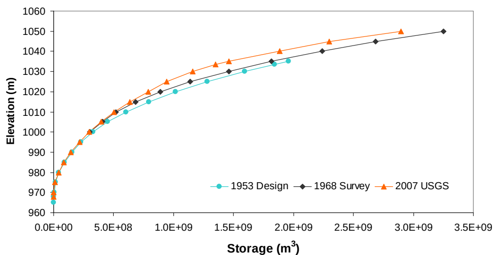
Figure 2-5. Storage–elevation relationships for the Kajakai Reservoir.
