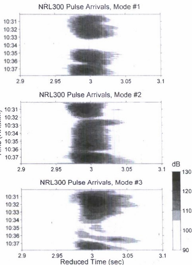
FIG. 13. (Color online) Broadband mode-filtered outputs of the received NRL300 pulses on the WHOI VLA during the truncated internal-wave event on August 20 in the SW06 experiment. The first three modes are shown, and a total of 110 pulses is analyzed. The mode intensities fluctuate in time.
