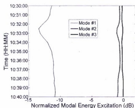
FIG. 11. Time series of theoretical estimates of the energy excitation of first three modes by the NRL300 source during the truncated internal-wave event shown in Fig. 9 on August 20.
