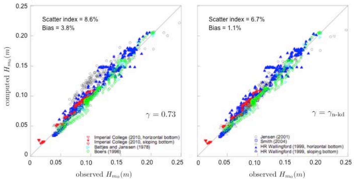
Figure 4 Scatter plots for predicted and observed significant wave height for a number of laboratory studies.
