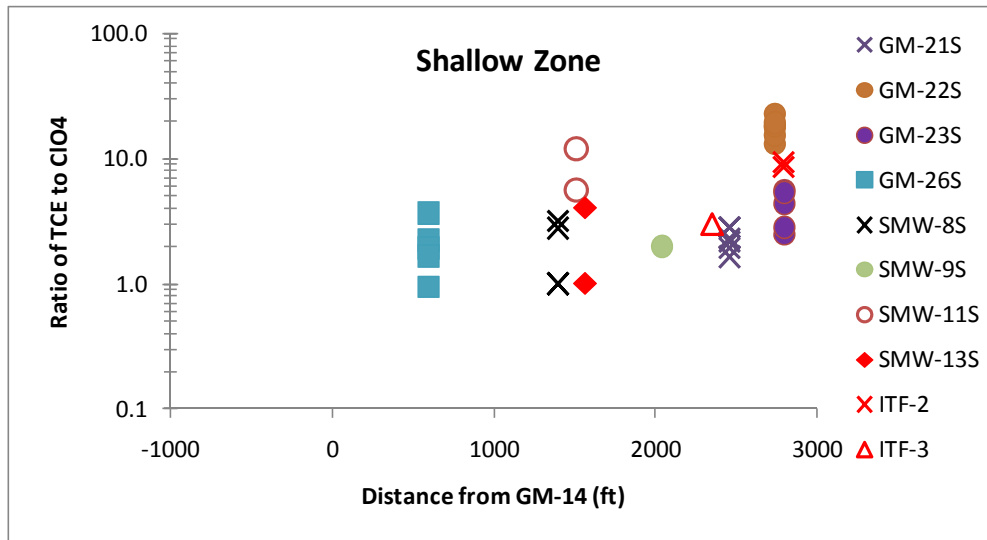
Figure 6-7b. Variation in TCE to ClO 4 Ratio in Shallow Zone Wells with Distance from Source
