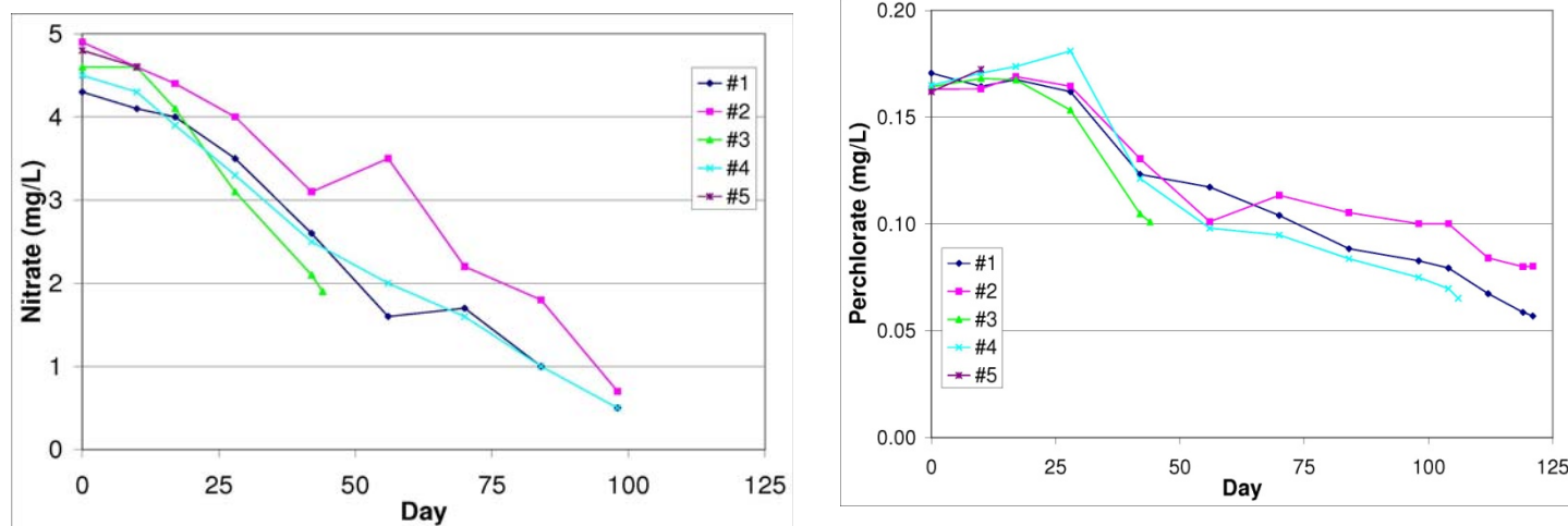
Figure 6-10. Concentrations of Nitrate (a) and Perchlorate (b) in Five Replicate Macrocosms
