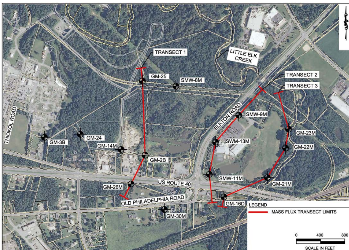
Figure 6-5. Mass Flux Calculation Transects
