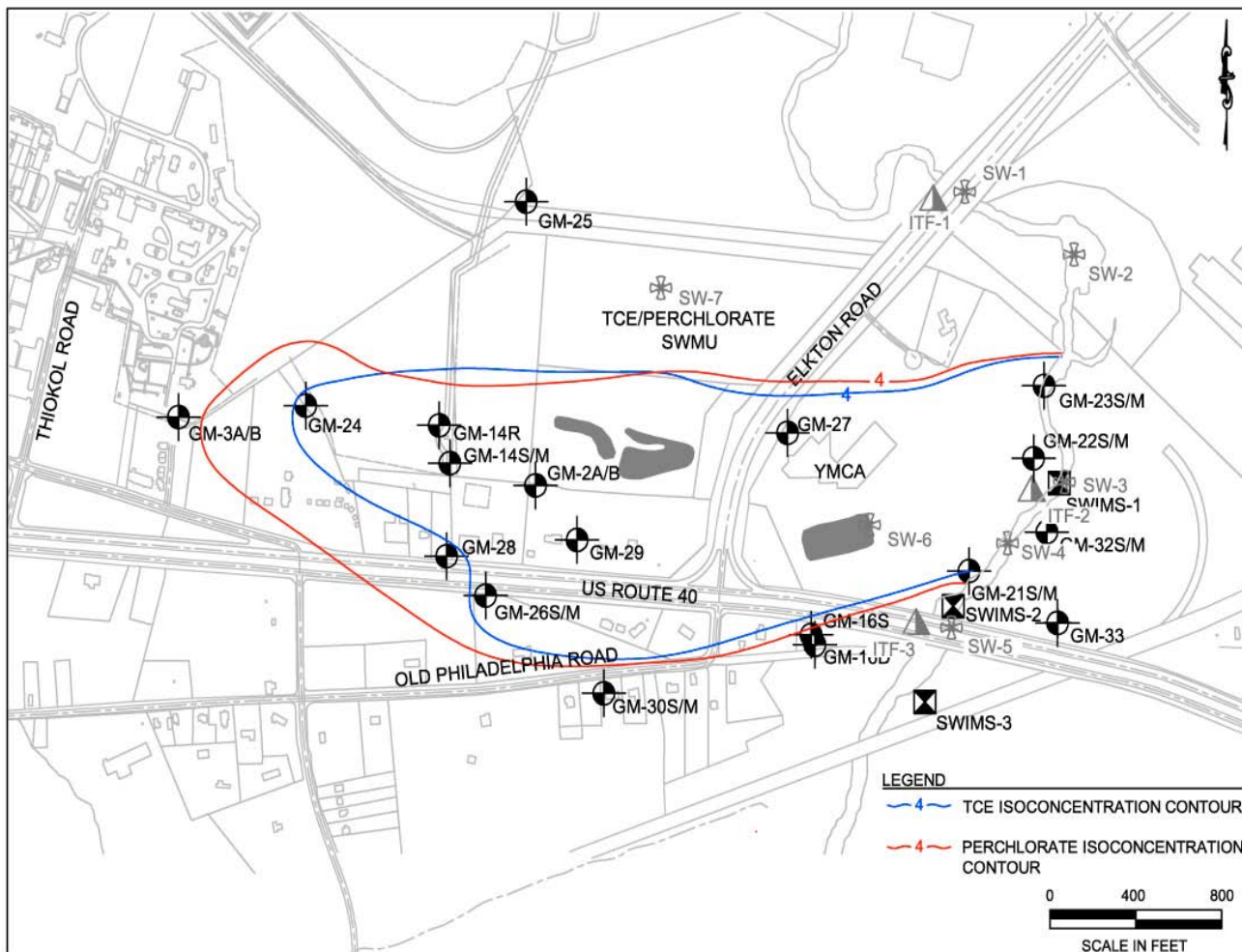
Figure 6-1. Baseline Perchlorate and TCE Delineation in the Intermediate Aquifer in May 2006
