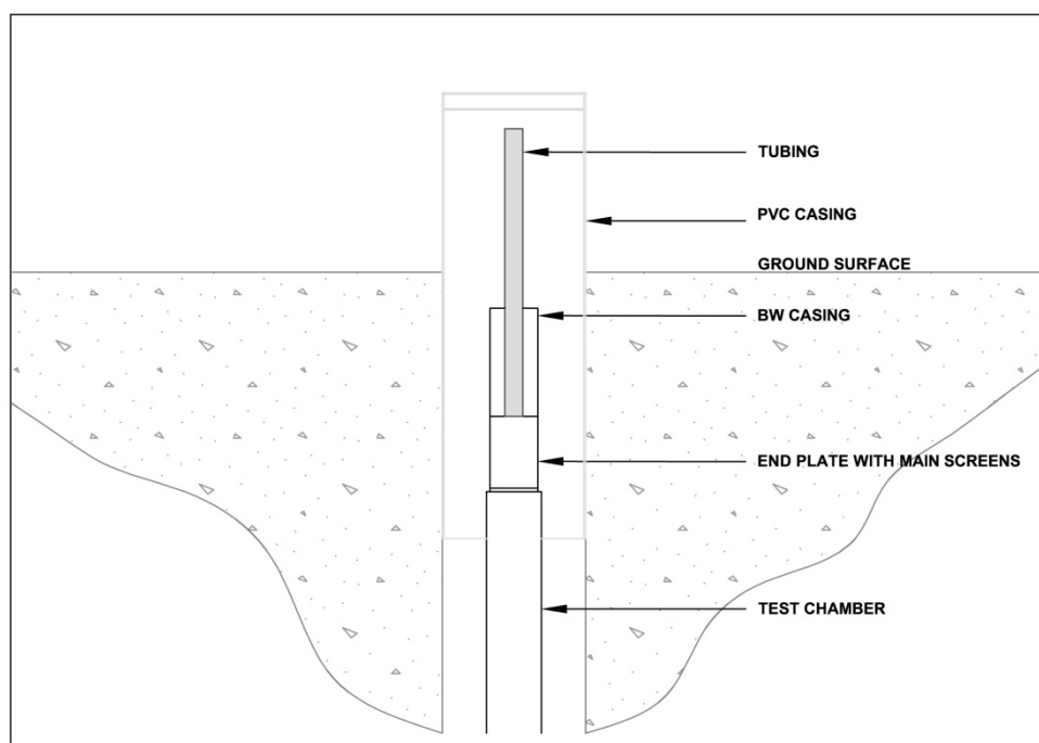
Figure 3-9. General Design of In Situ Columns
