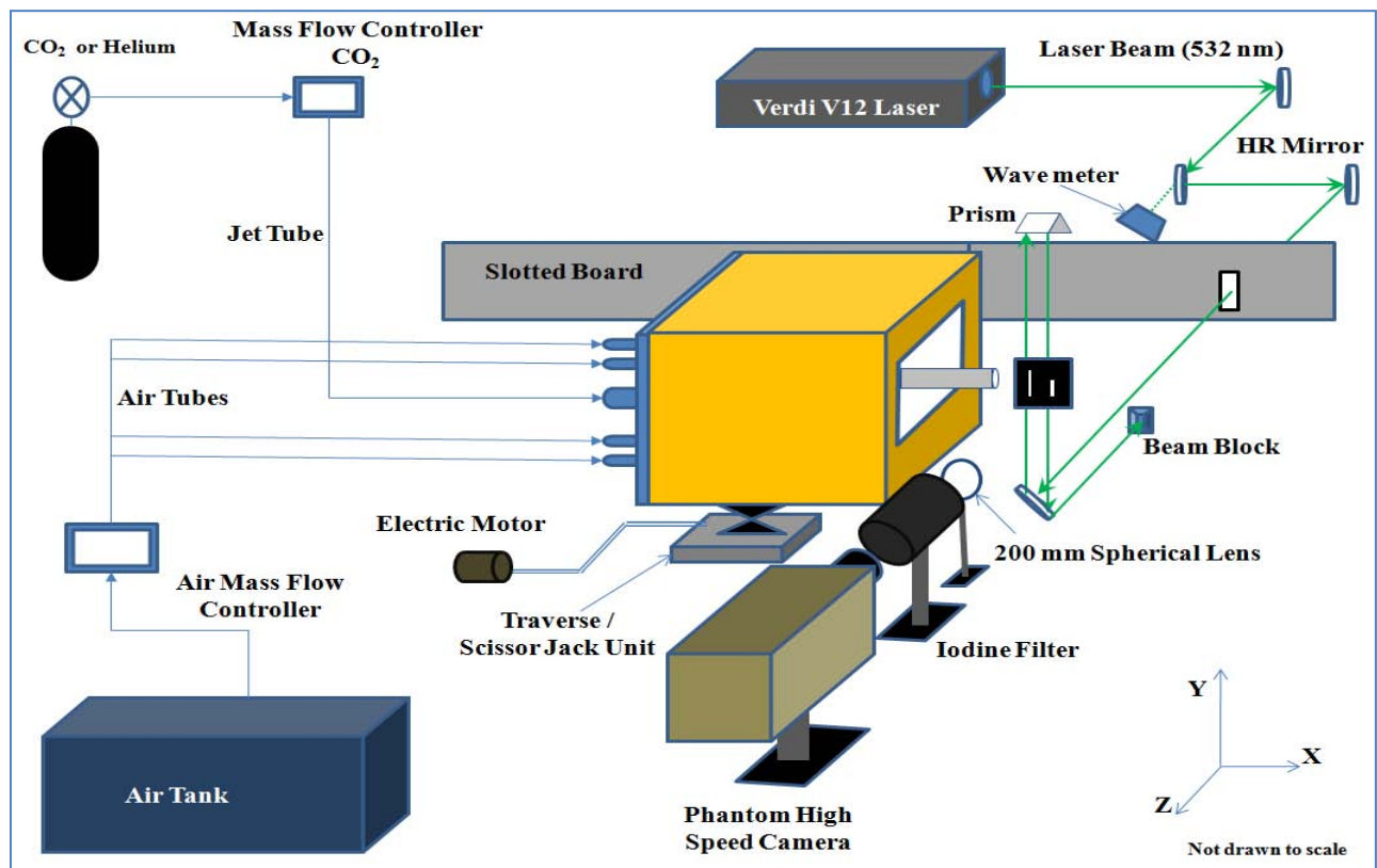
Figure 33. Diagram of Horizontal Buoyant Jet Set Up
