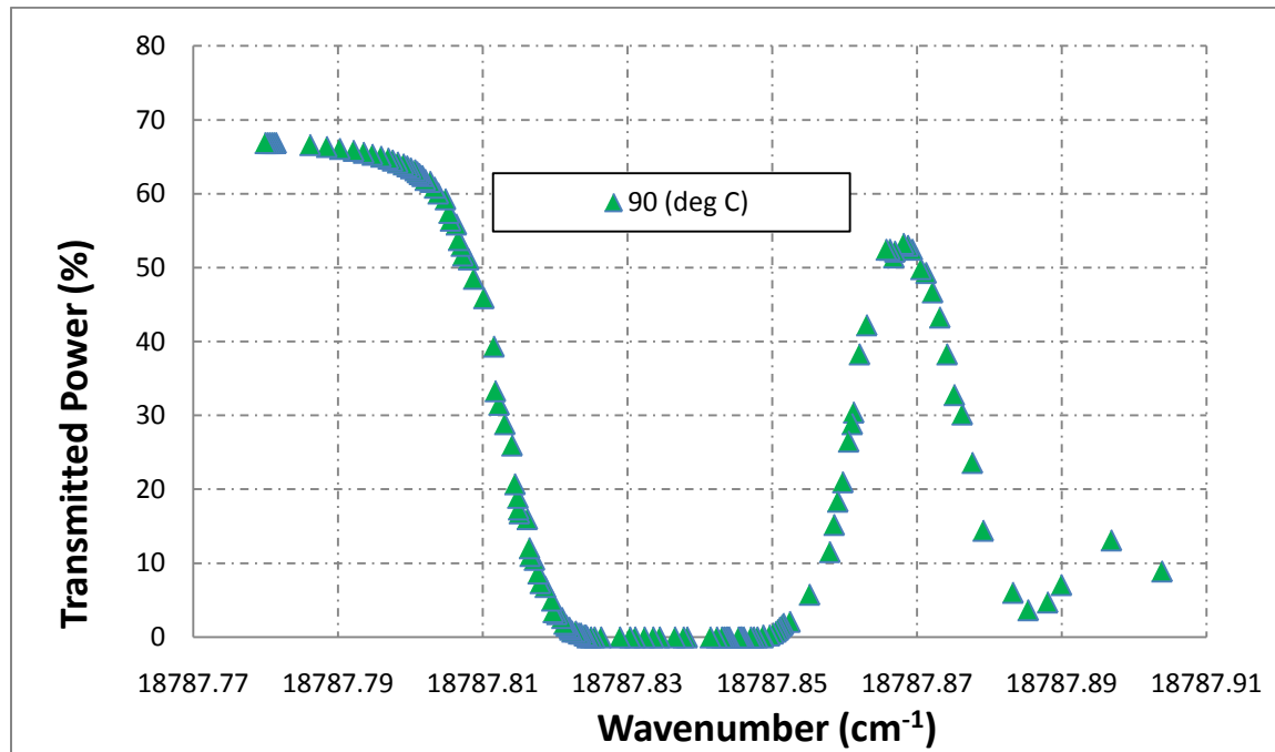
Figure 62. Investigation of the Upper End on the Absorption Well
