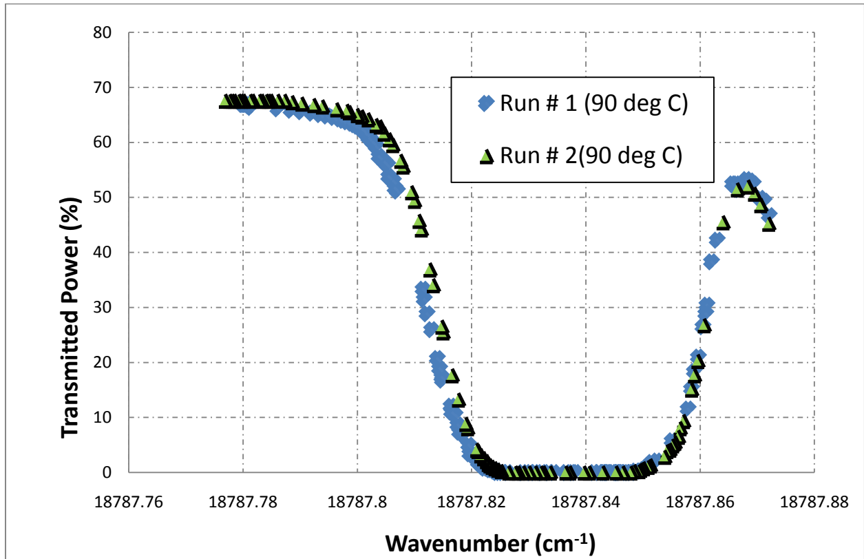
Figure 55. Repeatability Test of the Transmitted Power of the Filter at 90 °C
