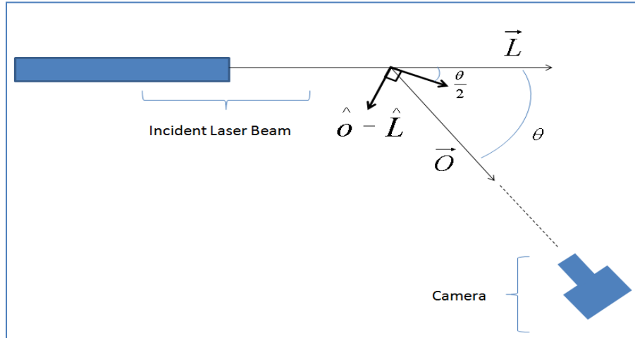
Figure 4. Diagram of a Typical Filtered Rayleigh Scattering Set Up (as inspired by Miles et al. 's figure)
