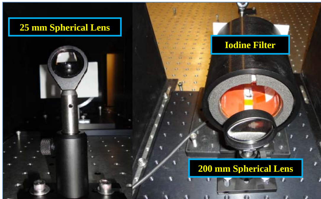
Figure 24. Spherical Lenses
