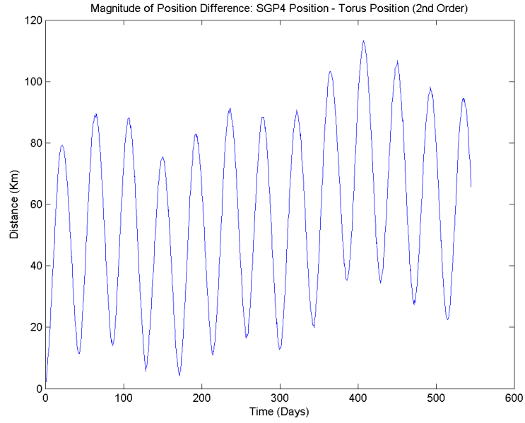
Figure 27: Error Magnitude: SGP4 Position - Torus Position, 2nd order Q_i
