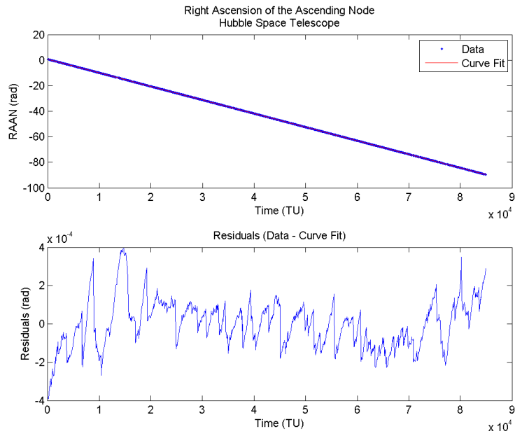
Figure 18: RAAN Data for the HST
