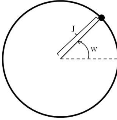
Figure 6: Diagram of a One-Dimensional Torus
