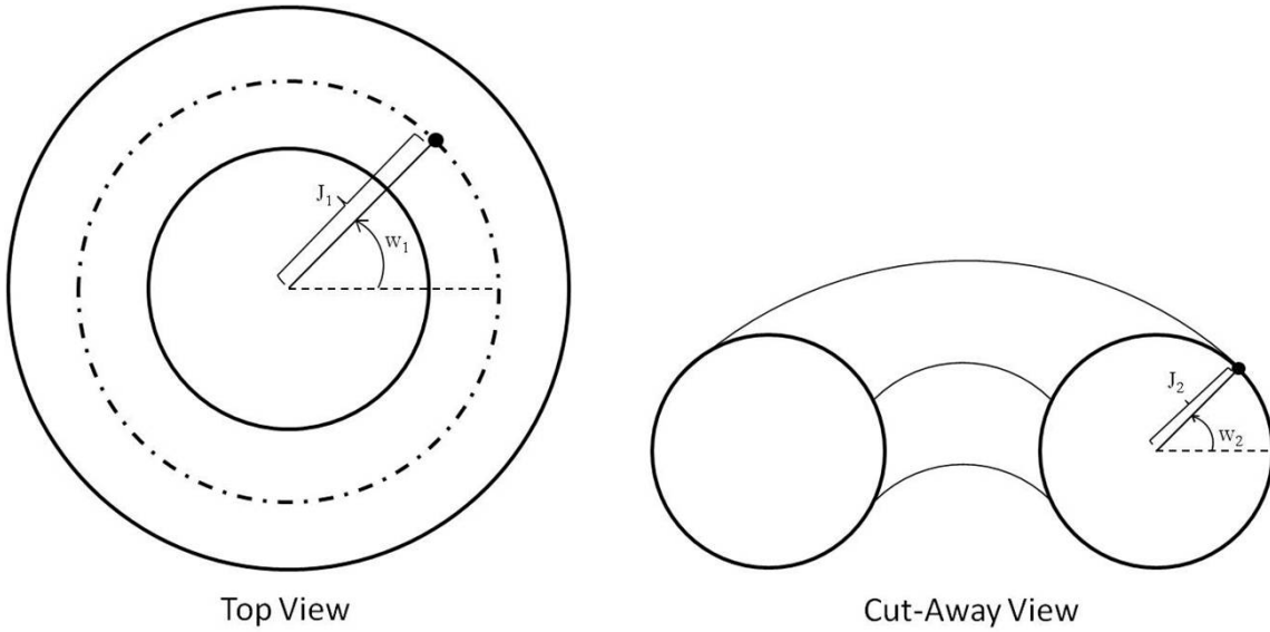
Figure 7: Diagram of a Two-Dimensional Torus
