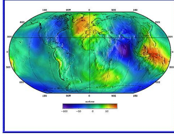
Figure 5: Visual Representation of EGM96 [10]
