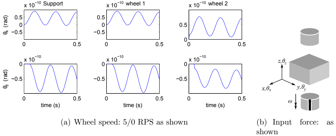
Figure 19: System demonstrating backward whirl
