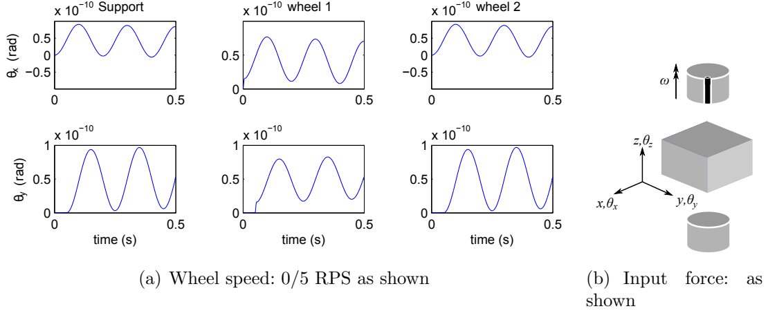
Figure 18: System demonstrating forward whirl
