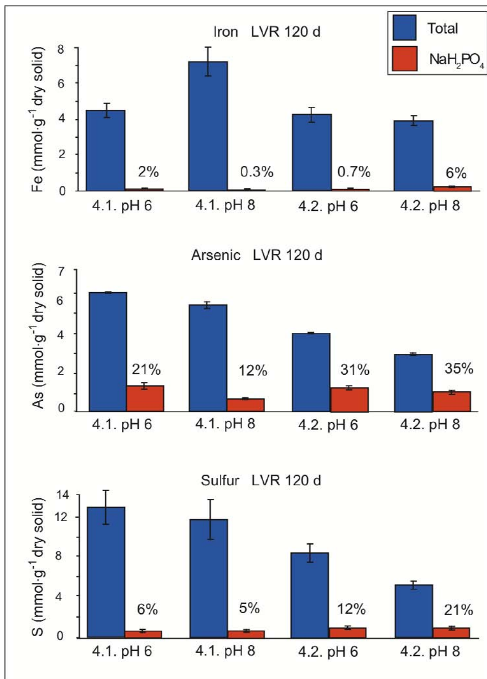
Figure 7. Extracted concentrations of Fe, As, and S compared to total concentrations from measurement of digested solids for LVR precipitates after 120 d of aging. Extraction solution was 0.005 M \text{NaH}_2\text{PO}_4 . Concentrations normalized to total dry weight of solids.
