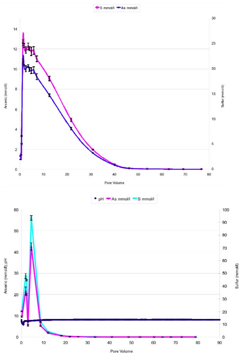
Figure 11. Total As and S in effluent solution in flow-through column dissolution experiments for amorphous \text{As}_2\text{S}_3(\text{s}) packed in an inert quartz matrix. Top: Influent solution: DO = 94%; pH 8 (Tris buffer). Bottom: Influent solution: DO = 0%; pH 8 (Tris buffer).
