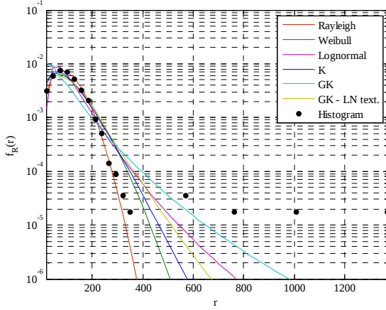
Figure 4. Amplitude PDF for RC 76 and azimuth -11^\circ .
