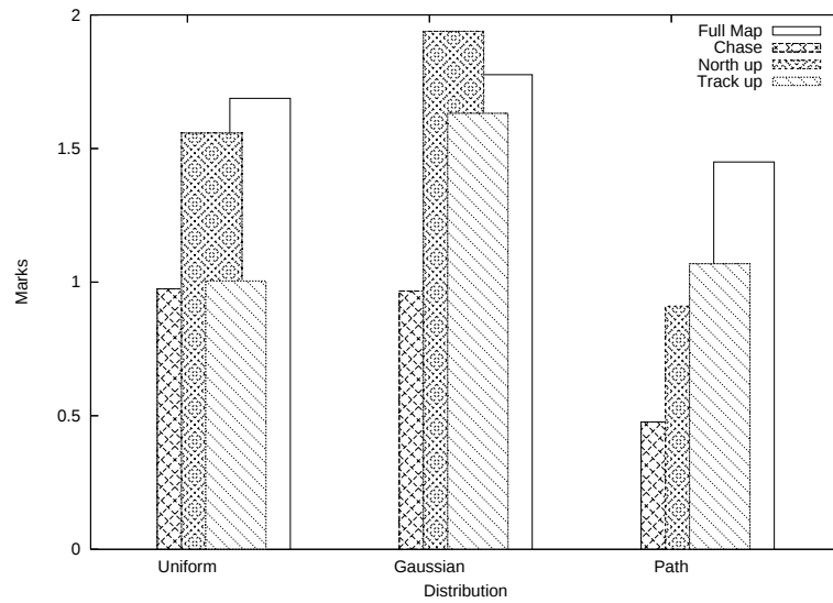
Figure 5.11: Redundant marks
