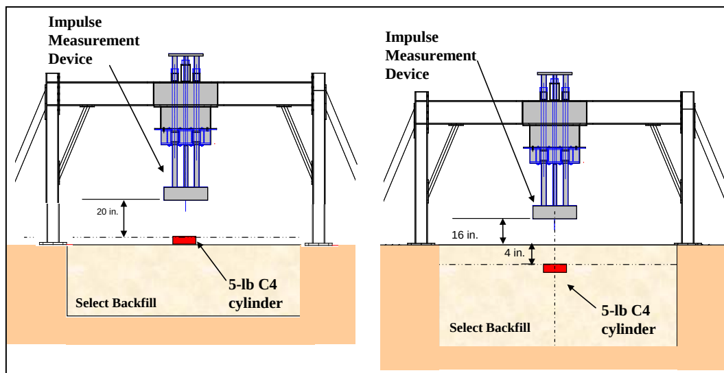
Figure 1. Example layouts for the IMD experiments.
