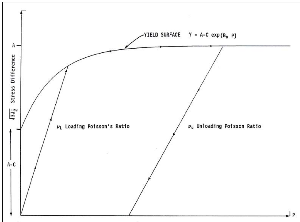
Figure 2. Model for simple HEP deviatoric behavior.
