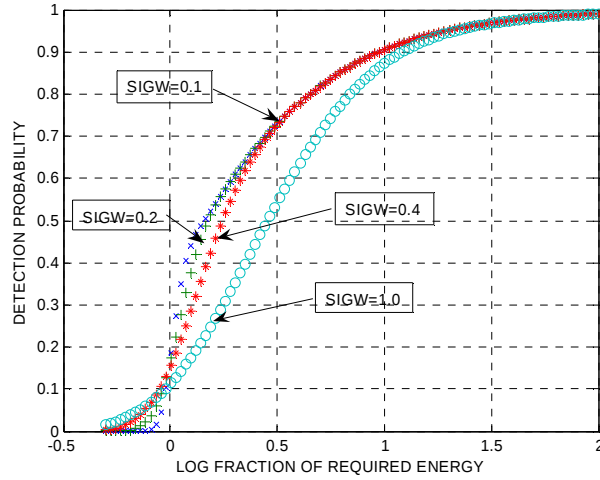
Figure 1. Detection probability for a Swerling I target as a function of nominal energy required for detection in atmospheric turbulence characterized by different values of \sigma_w (SIGW).
