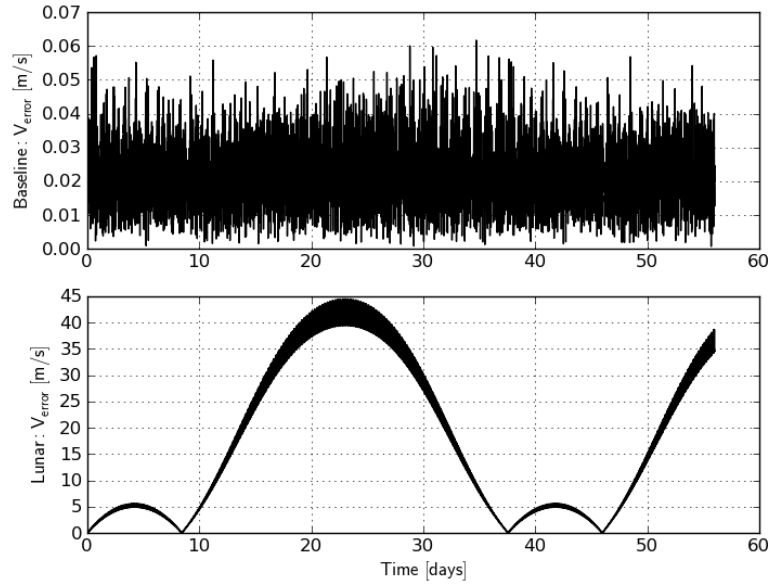
Figure 61: Total Velocity Error for Reference Torus and Perturbed Motion for Baseline and Lunar Cases
