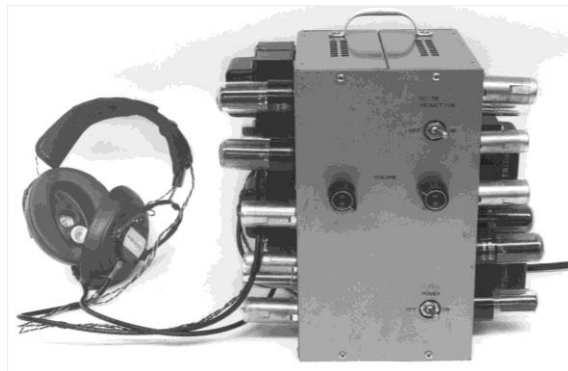
Figure 1. Active Noise Reduction Headset and Electron Tube Electronics circa 1957
