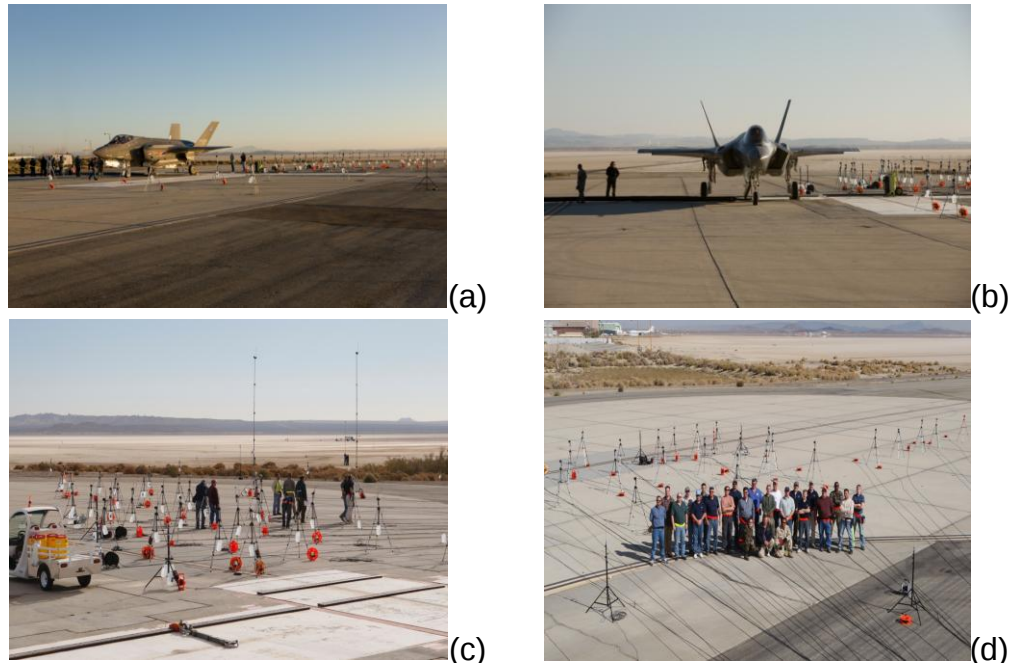
Figure 9. F-35 Lightning II Ground Run-Up Noise Measurement
