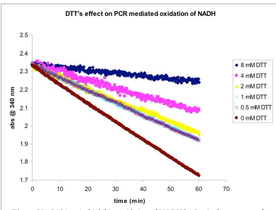
Figure 25. Dithiotreitol inhibits oxidation of NADH by Pcr in the presence of 100 \mu\text{M} perchlorate
