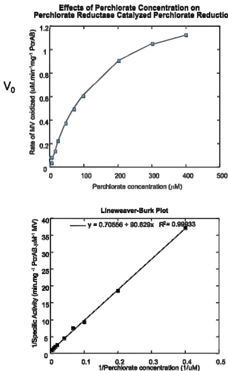
Figure 7. Effects of perchlorate concentration on perchlorate reductase catalyzed perchlorate reduction
