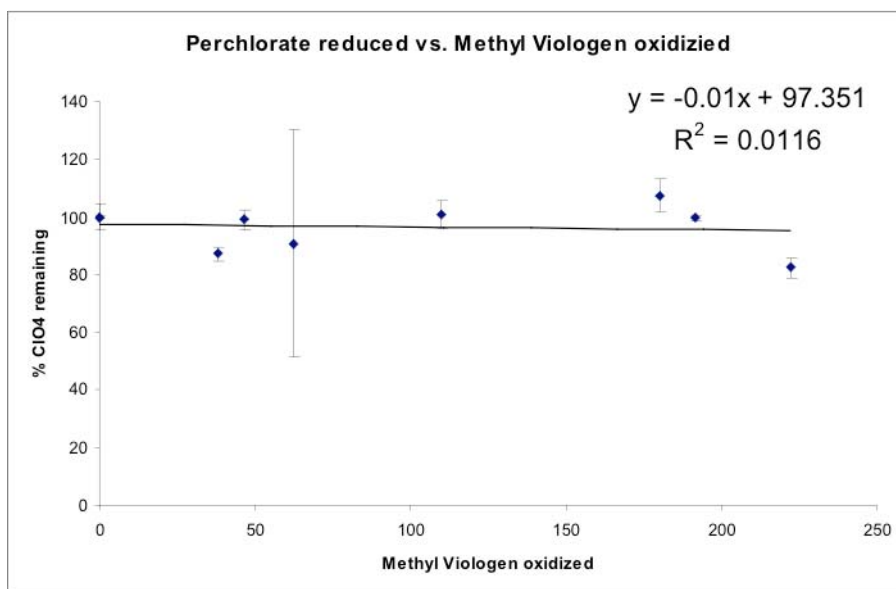
Figure 16. The perchlorate remaining following an incubation with perchlorate reductase and reduced methyl viologen.
