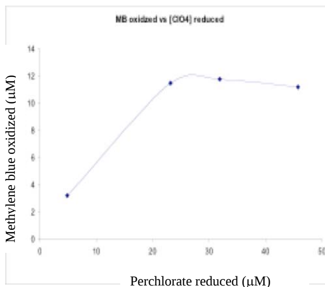
Figure 22. Methylene blue oxidized by perchlorate reductase in the presence of various concentrations of perchlorate
