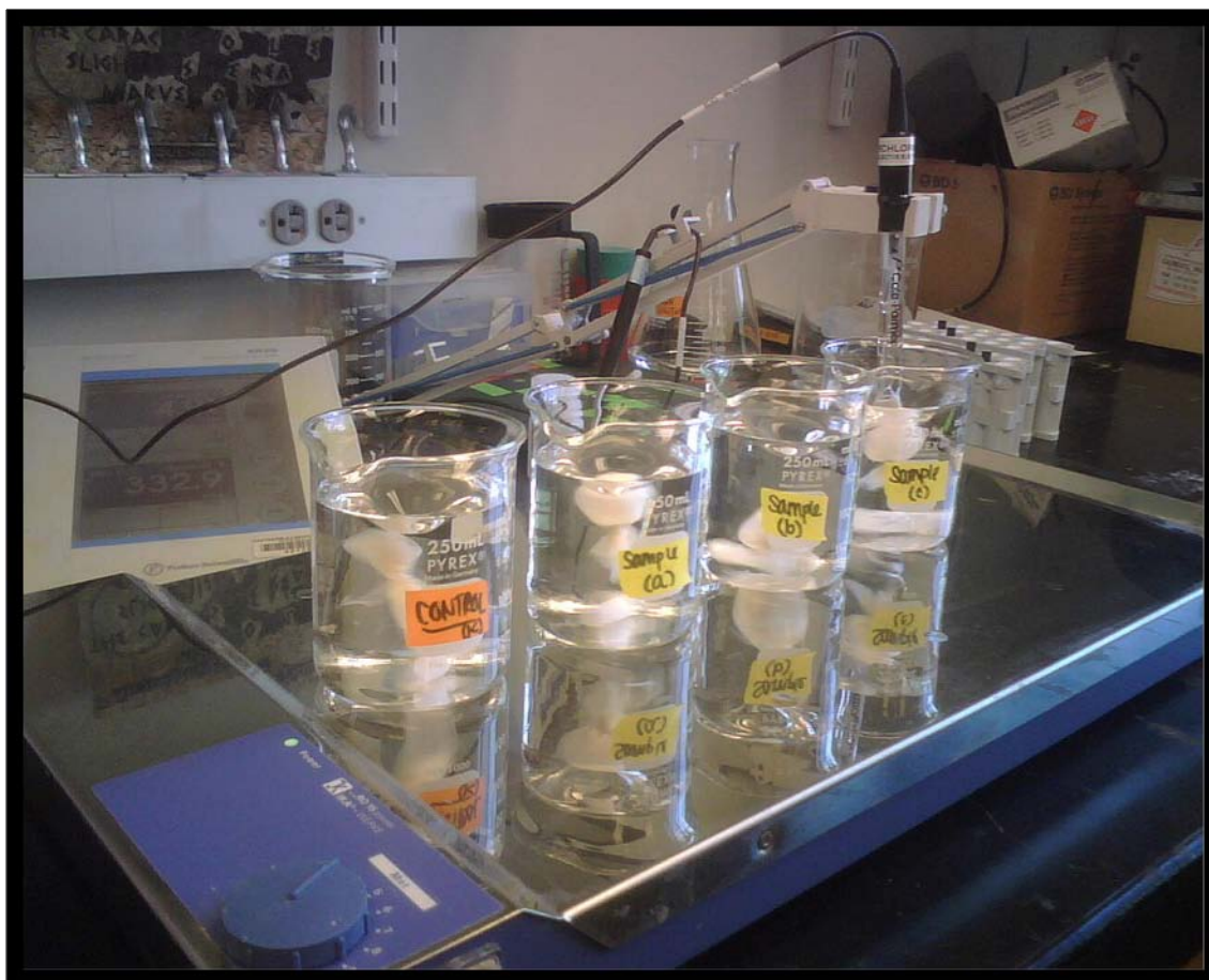
Figure 45. Extraction of perchlorate from 200ml samples using 1g of DTAB treated SDVB resin in teabags.
