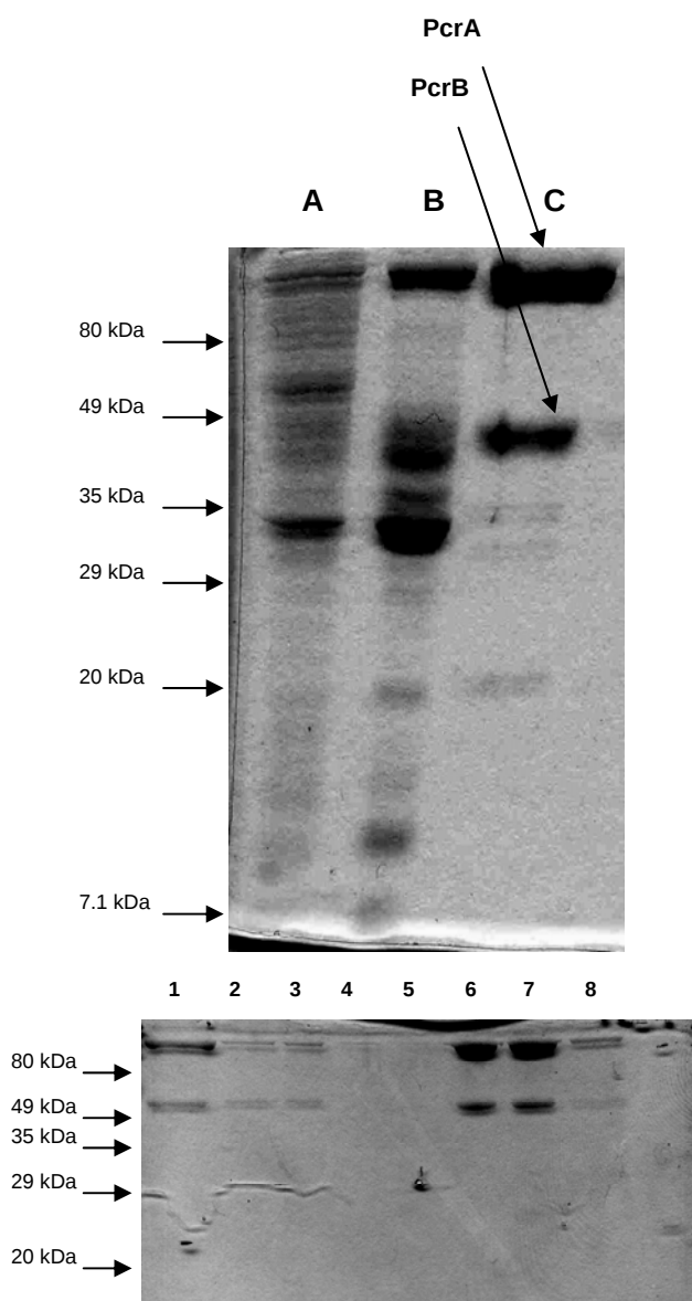
Figure 32. Purification of Perchlorate reductase using a streamlined protocol: Samples were analyzed on a 12% acrylamide gel, and stained using Coomassie G-250.
