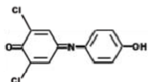
Dichlorophenol indophenol, E^{0'} = +217 mV (DCPIP)
