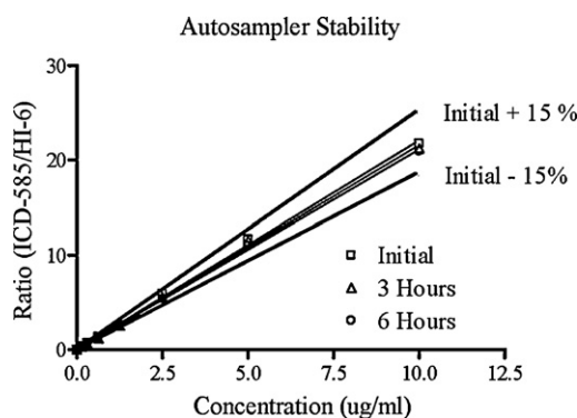
Fig. 6. Autosampler stability: plasma samples were prepared and placed in the autosampler. The prepared samples were analyzed immediately ( n=6 , square) and again at 3 ( n=6 , triangle) and 6 h ( n=4 , circle). Also shown are calculated curves corresponding to \pm 15\% (solid black lines) of the initial analysis.
