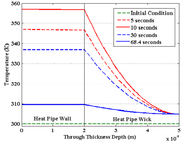
Figure 13: Temperature distribution through the heat pipe
