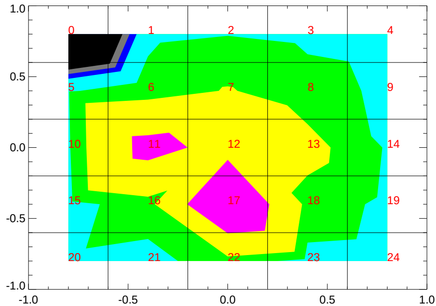
Figure 5-4 – Monostatic QC contour plot for example anomaly.
