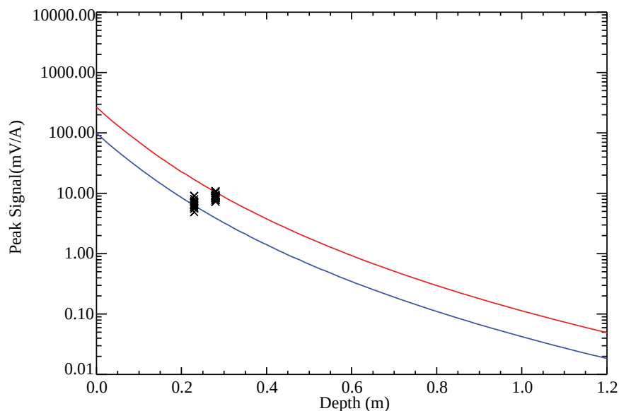
Figure 7-1 – Peak signals compared with response curve for a 60-mm mortar.
