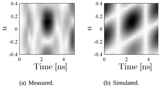
Fig. 5. Measured (a) and simulated (b) transmit signals for the MC signals \hat{\Upsilon}_{0,b,n}^{MC1} and \hat{\Upsilon}_{1,b,n}^{MC2} . The measured and simulated transmit signals do not agree because the model does not adequately represent the signals output by the TRCs.
