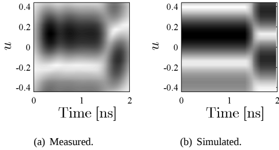
Fig. 4. Measured (a) and simulated (b) transmit signals for the Barker sequence \hat{\Upsilon}_0^{PC1} , and the Hadamard sequence \hat{\Upsilon}_1^{PC2} . The measured and simulated transmit signals are in fair agreement.
