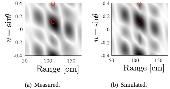
Fig. 8. Measured (a) and simulated (b) range-angle plots for the MC signals \hat{\Upsilon}_{0,b,n}^{MC1} and \hat{\Upsilon}_{1,b,n}^{MC2} using the modified signal model. The target locations are marked on the plots with circles. The measured and simulated range-angle plots are in fair agreement.
