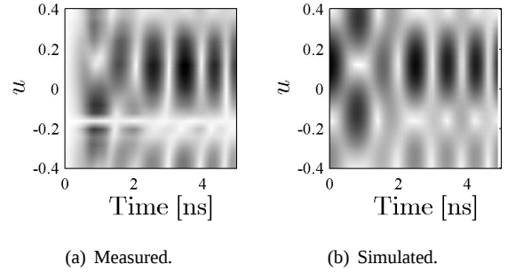
Fig. 7. Measured (a) and simulated (b) transmit signals for the MC signals \hat{\Upsilon}_{0,b,n}^{SC1} and \hat{\Upsilon}_{1,b,n}^{LFM1} using the modified signal model. The measured and simulated transmit signals are in fair agreement.
