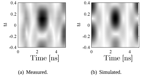
Fig. 6. Measured (a) and simulated (b) transmit signals for the MC signals \hat{\Upsilon}_{0,b,n}^{MC1} and \hat{\Upsilon}_{1,b,n}^{MC2} using the modified signal model. The measured and simulated transmit signals are in fair agreement.
