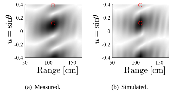
Fig. 9. Measured (a) and simulated (b) range-angle plots for the SC signal \hat{\Upsilon}_{0,b,n}^{SC1} and the LFM signal \hat{\Upsilon}_{1,b,n}^{LFM1} using the modified signal model. The target locations are marked on the plots with circles. The measured and simulated range-angle plots are in fair agreement.
