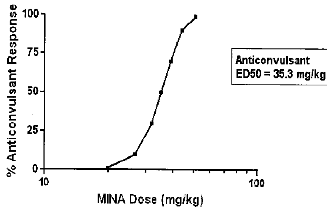
Figure 4. Anticonvulsant dose-dependent effect curve for MINA when administered 1 min after sarin ( 2 \times LD_{50} , sc) challenge. Note the X-axis is in log units.
