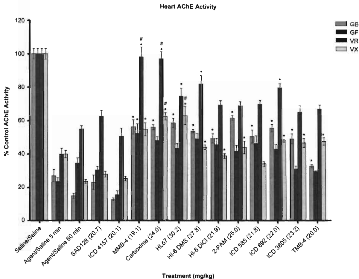
Figure 5. Effects of nerve agent and oxime treatments on heart AChE activity in the guinea pig. Saline, SAD128, ICD 4157, MMB-4, carboxime, HLö7, HI-6 DMS, HI-6 DiCl, 2-PAM, ICD 585, ICD 692, ICD 3805, or TMB-4 was given intramuscularly 5 min after a 1.0 LD 50 subcutaneous dose of GB, GF, VR, or VX. The non-oximes (SAD128 and ICD 4157) served as negative controls of enzyme reactivation. Samples were collected at 60 min after nerve agent administration. Total AChE activity was expressed as mean \pm SEM (% of control group) with 6–8 animals per group. 'Agent/Saline 5 min' data were taken from Shih et al. (2005). * Significantly different from nerve agent at 60 min, p < 0.05 . # Significantly different from 2-PAM, p < 0.05 . (See colour version of this figure online at www.informahealthcare.com/txm ).
