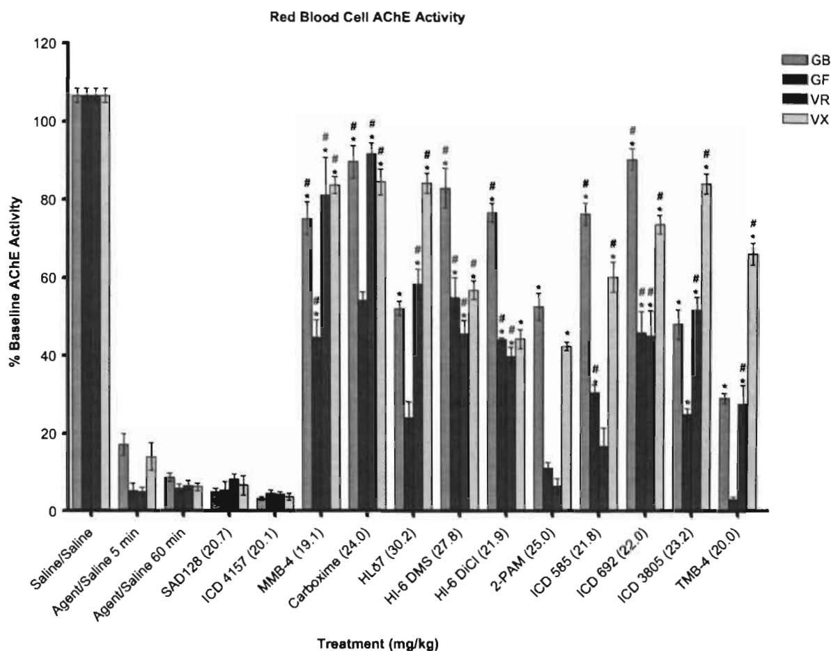
Figure 2. Effects of nerve agent and oxime treatments on red blood cell (RBC) AChE activity in the guinea pig. Saline, SAD128, ICD 4157, MMB-4, carboxime, HLö7, HI-6 DMS, HI-6 DiCl, 2-PAM, ICD 585, ICD 692, ICD 3805, or TMB-4 was given intramuscularly 5 min after a 1.0 LD 50 subcutaneous dose of GB, GF, VR, or VX. The non-oximes (SAD128 and ICD 4157) served as negative controls of enzyme reactivation. Samples were collected at 60 min after nerve agent administration. AChE activity in RBC was expressed as percentage of individual baseline AChE activity. The baseline AChE activity was obtained 1–3 days prior to experimental treatment. Total AChE activity was expressed as mean \pm SEM (% of control group) with 6–8 animals per group. 'Agent/Saline 5 min' data were taken from Shih et al. (2005). * Significantly different from nerve agent at 60 min, p < 0.05 . # Significantly different from 2-PAM, p < 0.05 . (See colour version of this figure online at www.informahealthcare.com/txm ).
