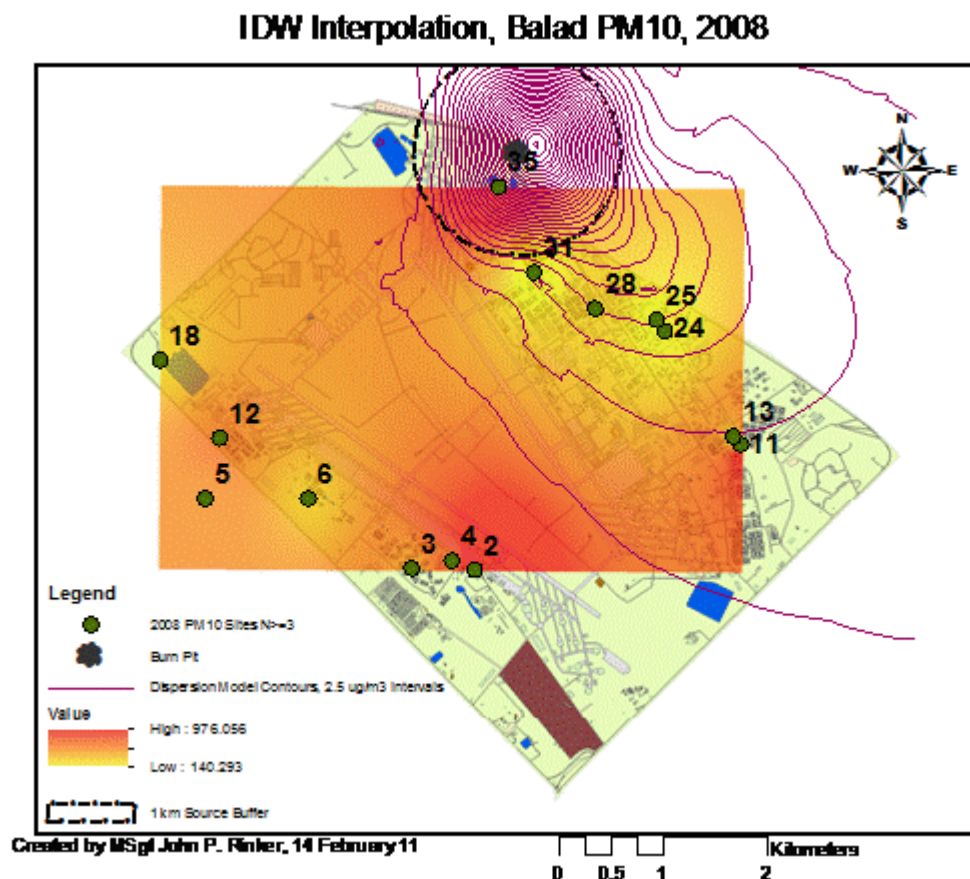
Figure 28: Inverse Distance Weighting Interpolation, Ambient PM10, Balad, 2008
