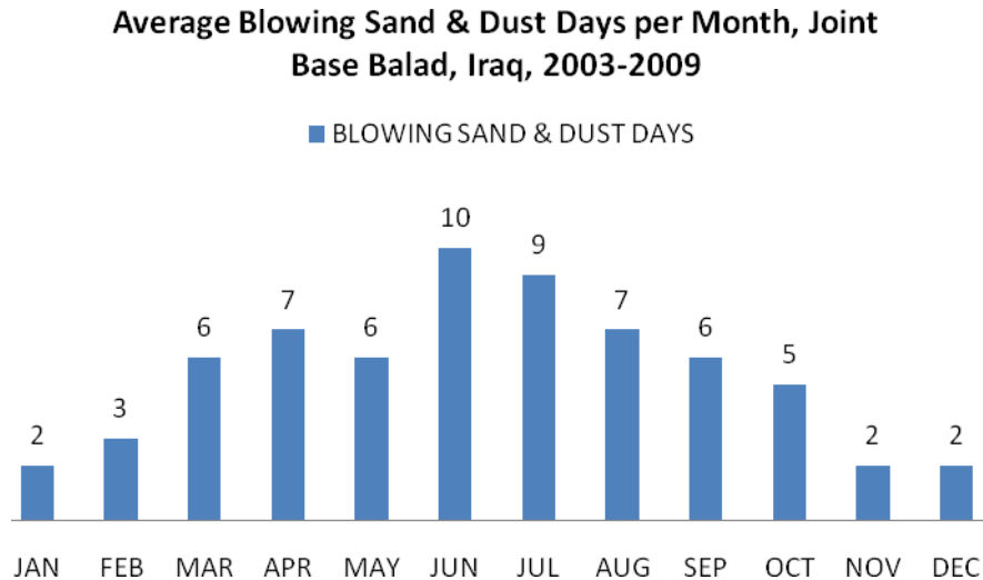
Figure 9: Average Monthly Dust Storm Frequency, Joint Base Balad (14WS, 2010)
