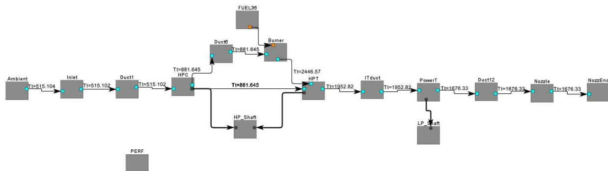
Figure 2. NPSS Model of a 50 shp Turboshaft Engine. HPC=High Pressure Compressor, HPT=High Pressure Turbine
