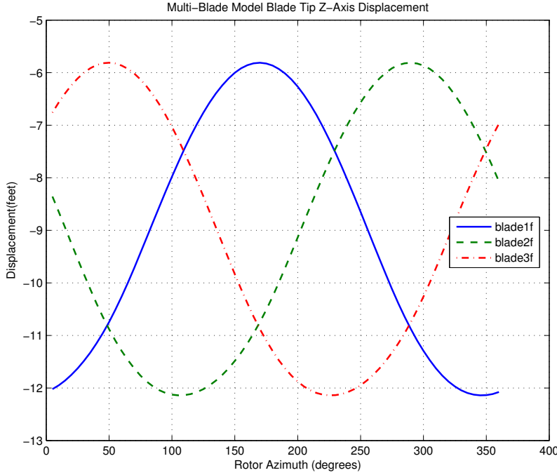
Figure 4.3: Multi-Blade Model Forward Rotor Blade Tip Displacements
