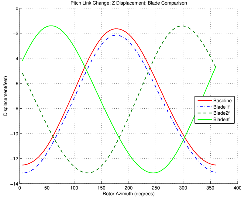
Figure 4.8: Testing Slide Input - Blade Tip Displacement Comparison
