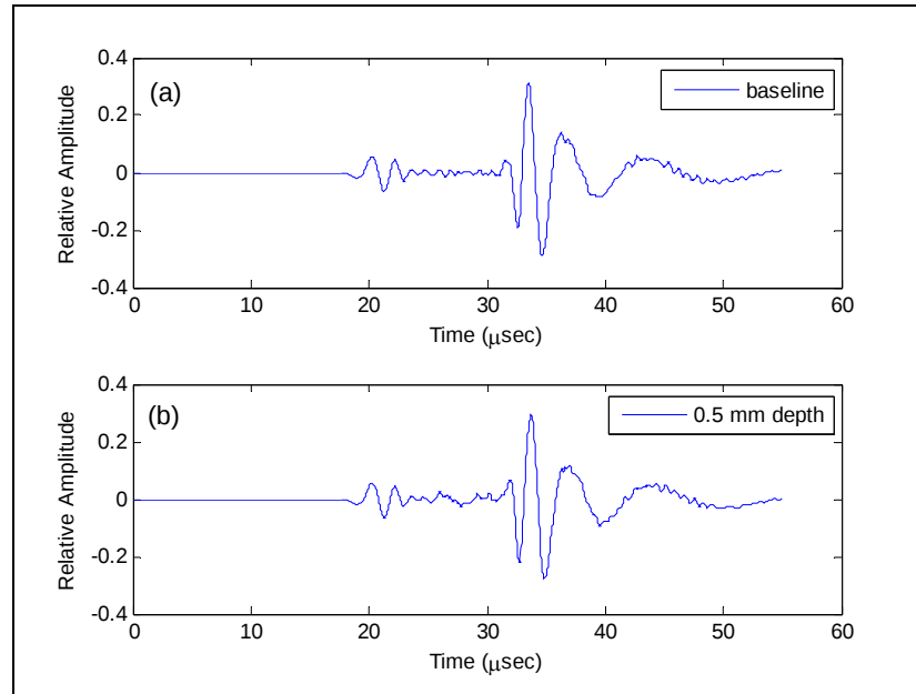
Figure 6. Simulated time-domain signal showing the primary symmetric and antisymmetric modes for (a) baseline signal without damage and (b) a notch with 0.5-mm depth. (Source signal was a sine exponential pulse.)
