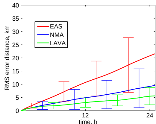
Fig. 11. Comparison of rms errors for drifter trajectories modeled using EAS-16 (red), NMA corrected (blue) and LAVA corrected (green) velocity fields. Time is measured from each drifter's launch. Error bars show \pm one standard deviation. (For interpretation of the references to colour in this figure legend, the reader is referred to the web version of this article.)
