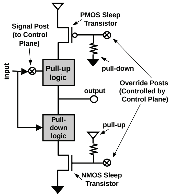
Figure 3: A circuit diagram of sleep transistors in the computation plane being used to remove power from a circuit.
