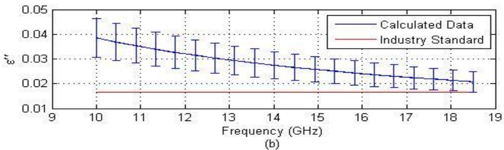
Figure 4-19: \epsilon_r for a 4.39mm thick sample of Plexiglas using circular plates with zero padding
