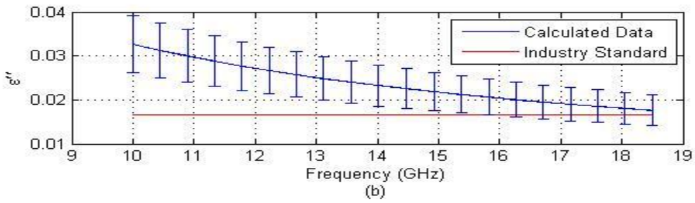
Figure 4-18: \epsilon_r for a 4.39mm thick sample of Plexiglas using circular plates with no zero padding
