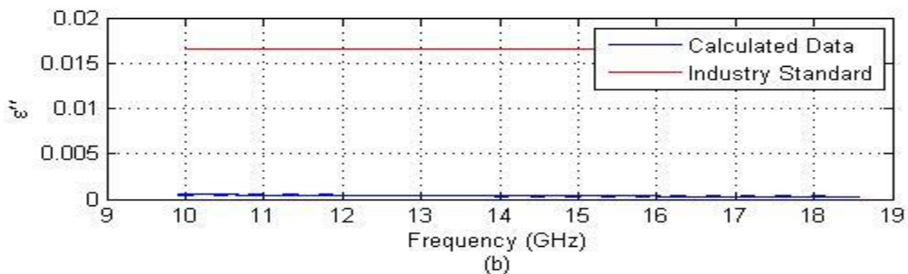
Figure 4-23: \epsilon_r for a 4.39mm thick sample of Plexiglas using square plates with zero padding
