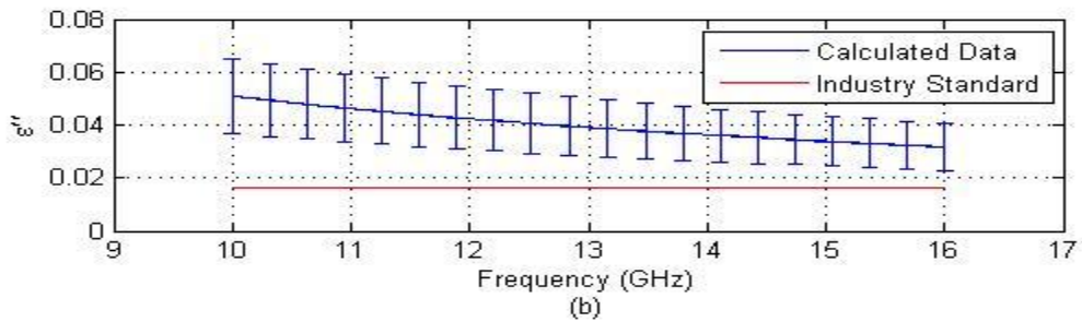
Figure 4-21: \epsilon_r for a 5.55mm thick sample of Plexiglas using square plates with zero padding
