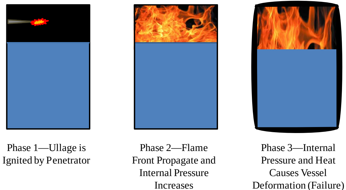
Figure 4-19: Phases of Fire Growth and Effects
