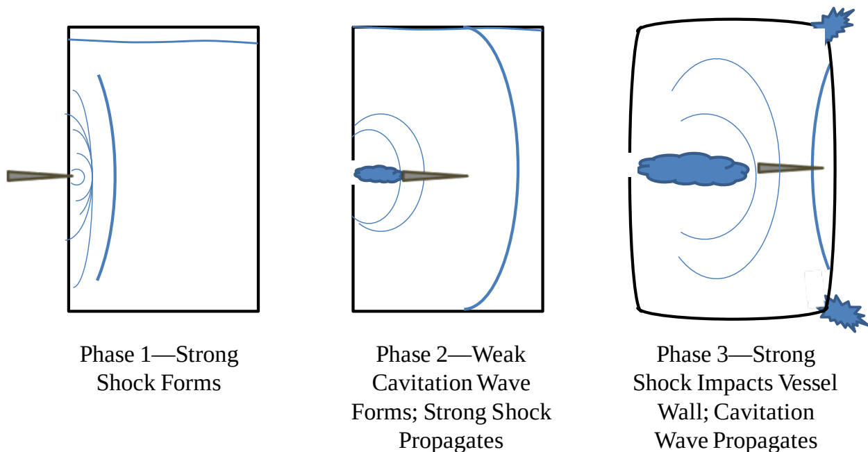
Figure 4-18: Phases of Hydrodynamic Ram
