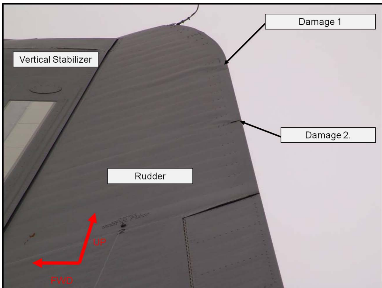
Figure 4-12: C-130J Vertical Stabilizer and Rudder Battle Damage, image courtesy of USAF C-130 Program Office [40]
