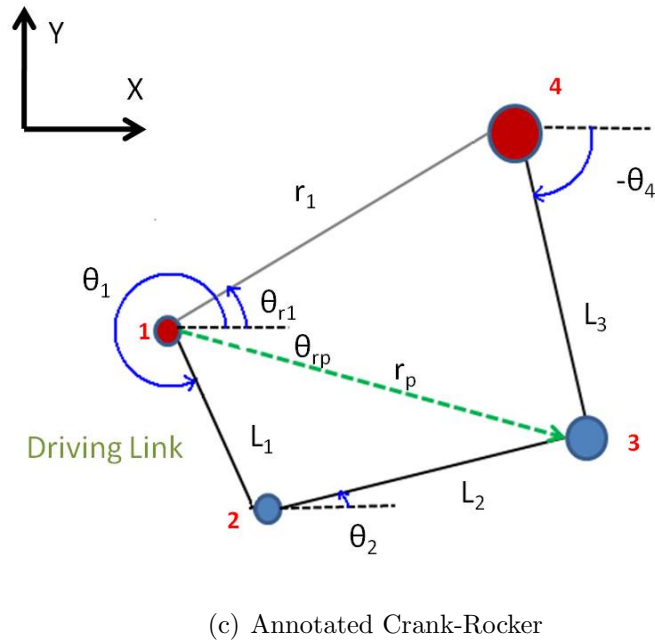
Figure F.2: Four Bar Flapper Visualization
