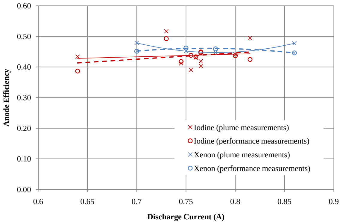
Figure 32: Comparison of plume and performance efficiencies at 250 volts discharge
