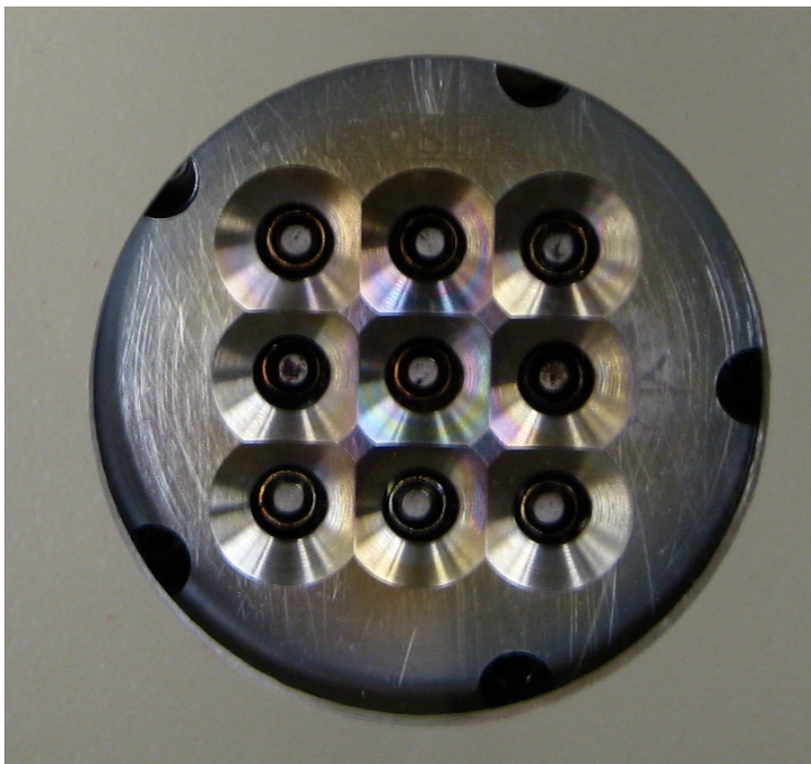
Figure 51. The thruster after operation. Note the discoloration on some of the emitter surfaces
