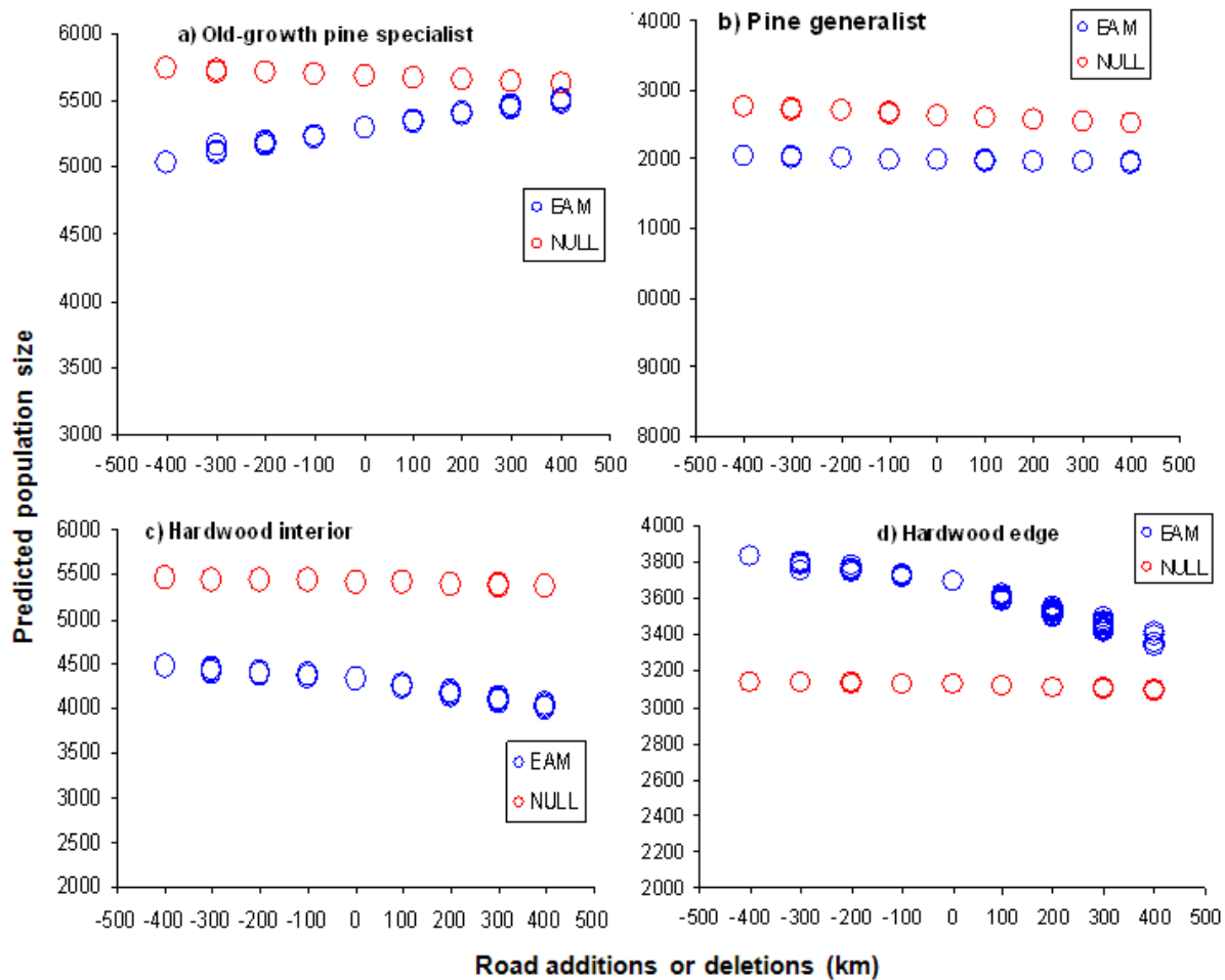
Figure. 24. Total predicted population sizes for four target “species” as roads are added and deleted throughout a model area on Ft. Benning. Predictions are shown for each scenario (10 replicates for each level of addition or deletion except 0 and -400) from the EAM and a NULL model that ignores edge and context.
