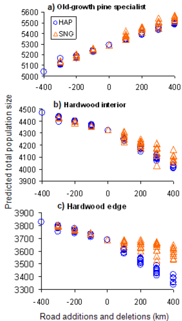
Figure 30. Total predicted populations for replicate scenarios representing different densities for roads drawn haphazardly (HAP) and roads drawn using StopNGo maps (SNG) for three "species".
