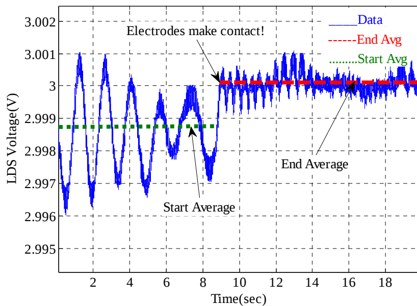
Figure 25. Electrode calibration
