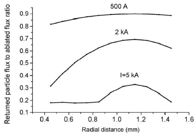
Figure 13. Particulate/Ablation ratio as function of current density, taken from Keidar [1]
