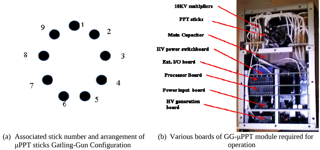
Figure 9. Gatling-Gun configuration and module
