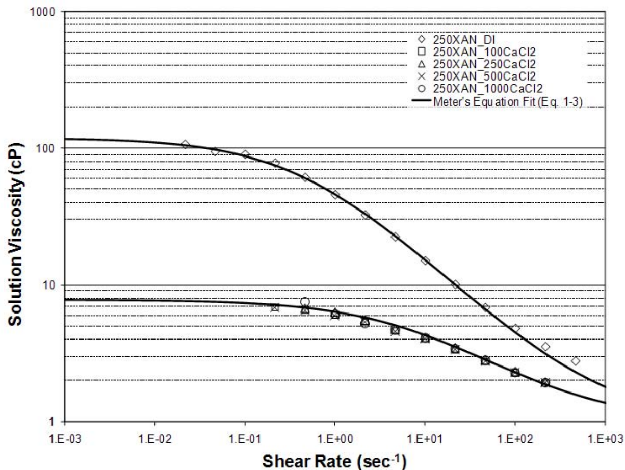
Figure 4-7: Viscosity/shear rate for 200 mg/L xanthan solutions as a function of \text{CaCl}_2 concentration.
