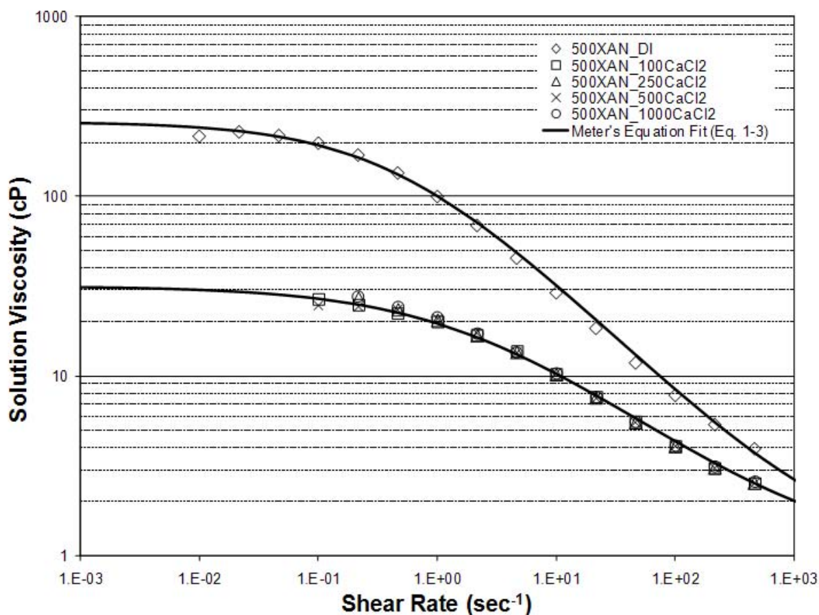
Figure 4-6: Viscosity/shear rate for 500 mg/L xanthan solutions as a function of \text{CaCl}_2 concentration.
