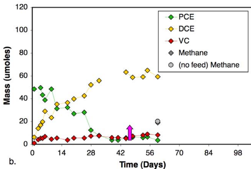
Figure 3-11: Total (liquid- + gas-phase) analyte mass versus time for xanthan e^- donor experiments (a) and nutrient medium e^- donor control experiments (b), from round one. Note that methane concentrations (shown in gray) refer to the right-hand y-axis for Figure 3.X.a only. Pink arrows indicate addition of methanol only. Data points referred to as “no feed Methane” are final methane measurements taken from “Viscosity control” (i.e., control experiments of either xanthan or nutrient medium containing microbes with no PCE feed). Data points shown are averages of three to four replicates (see Table 3-4).
