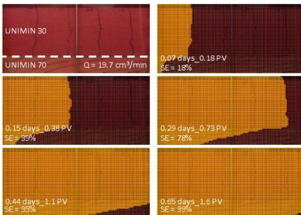
Figure 5-7: Polymer propagation within 2L_75%UNI30_25%UNI70 tank.
