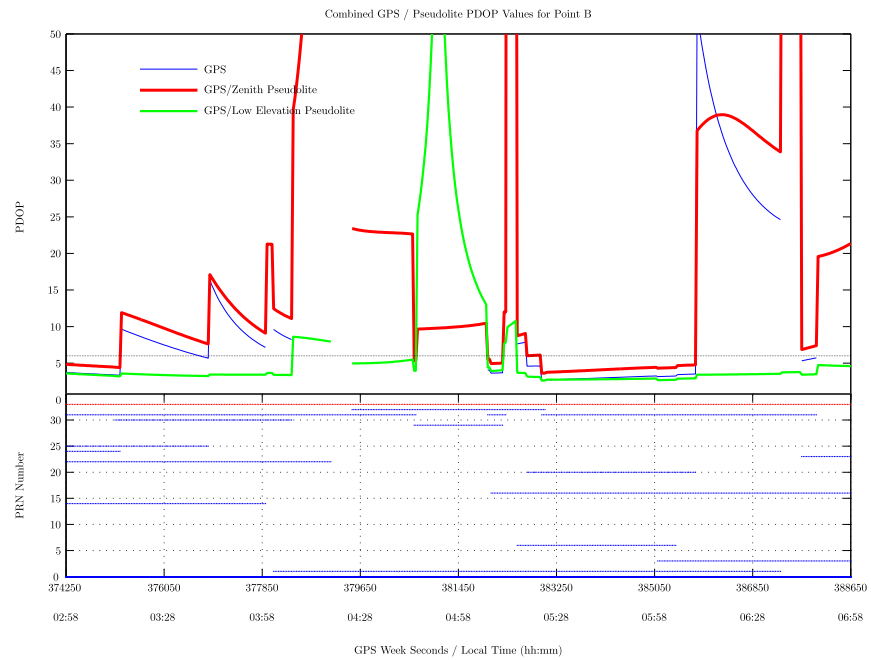
Figure 4.24: Combined GPS/Pseudolite PDOP values over Point B for 4 hours in UTZ type II.
