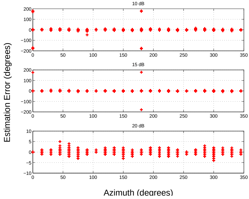
Figure B.2: f_c = 4 MHz Error Distribution vs. Azimuth for multiple SNR values using N_A = 8 individual feed points.
