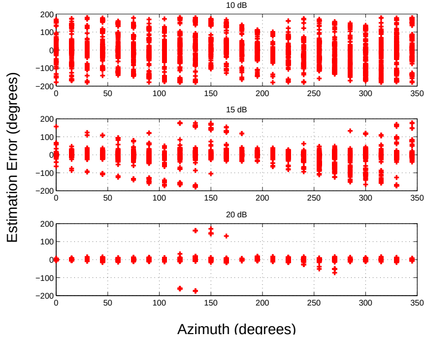
Figure B.8: f_c = 4 MHz Error Distribution vs. Azimuth for multiple SNR values using N_A = 8 feed points to synthesize a cube antenna pattern.
