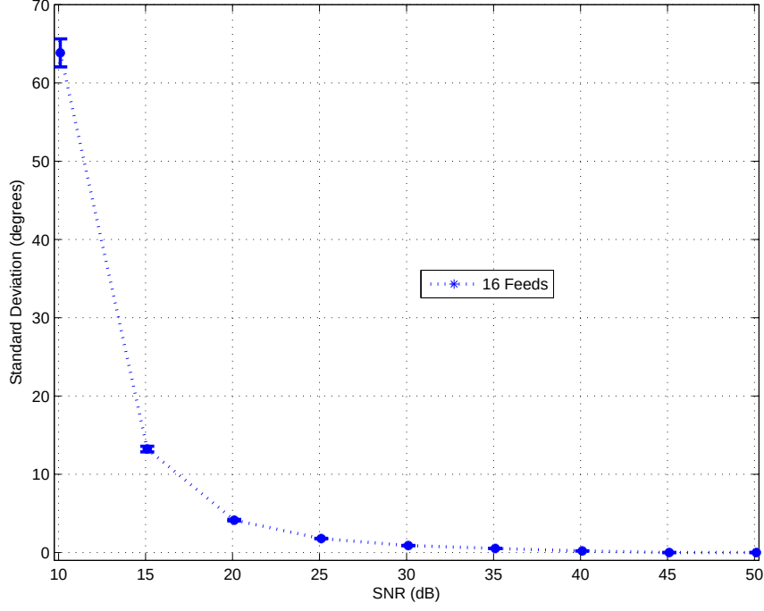
Figure 4.28: Standard deviation of AOA estimation error vs. SNR for a f_c = 4 MHz incident signal with 95% confidence intervals using N_A = 16 feed points to synthesize a cube antenna pattern.
