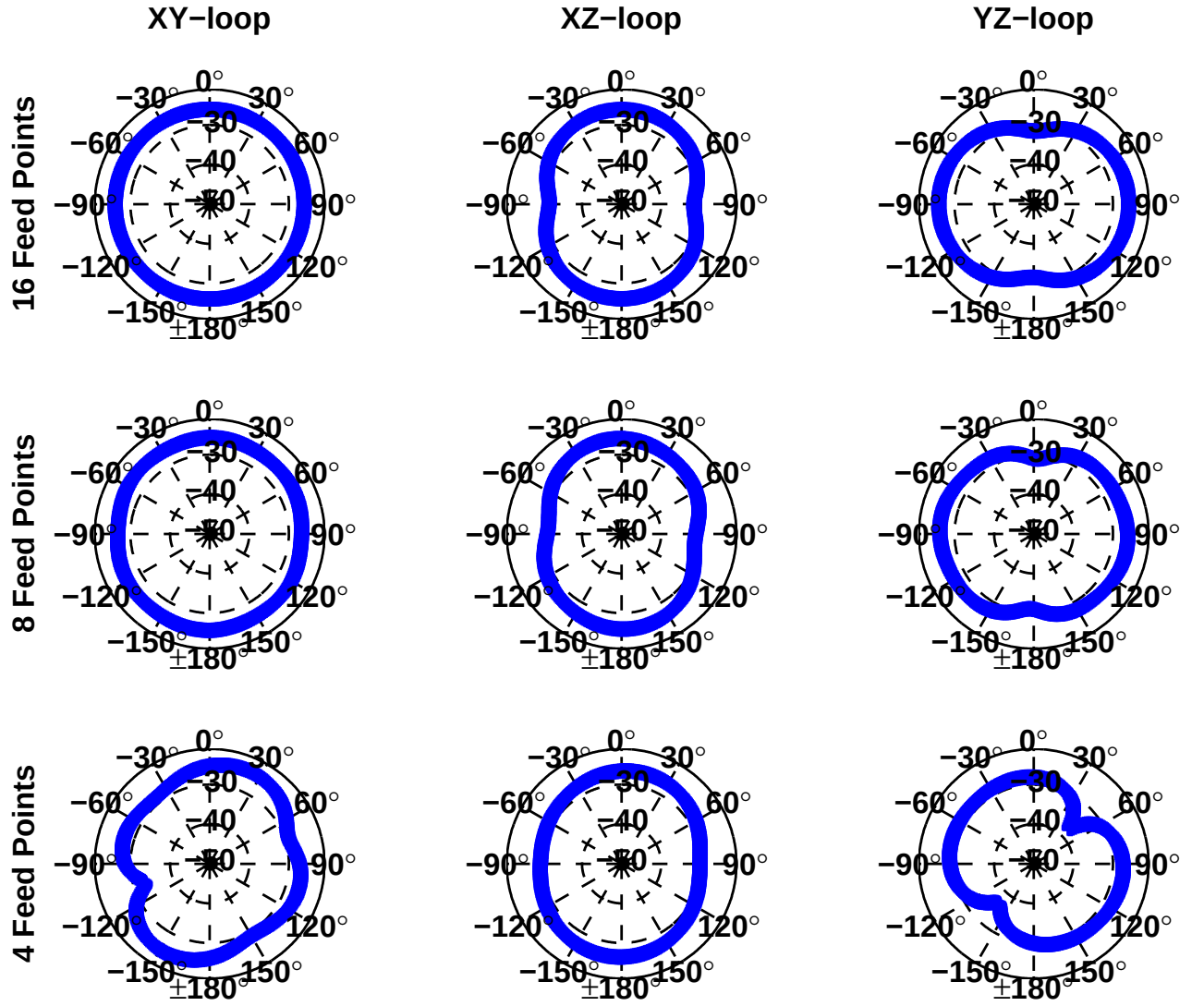
Figure A.3: f_c = 4 MHz synthesized cube antenna patterns. Each row contains all 3 loops for linear combinations of N_A = 16 , N_A = 8 , and N_A = 4 feed points.
