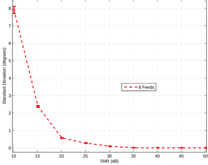
Figure 4.5: Standard deviation of AOA estimation error vs. SNR for a f_c = 4 MHz incident signal and N_A = 8 individual feed points with 95% confidence intervals.
