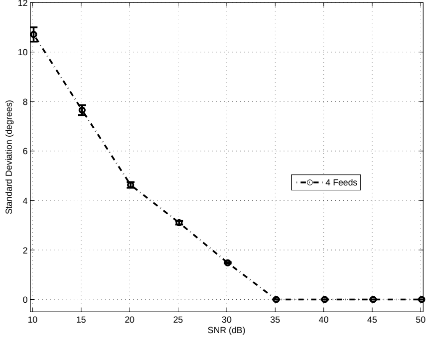
Figure 4.19: Standard deviation of AOA estimation error vs. SNR for an f_c = 11 MHz incident signal and N_A = 4 individual feed points with 95% confidence intervals.
