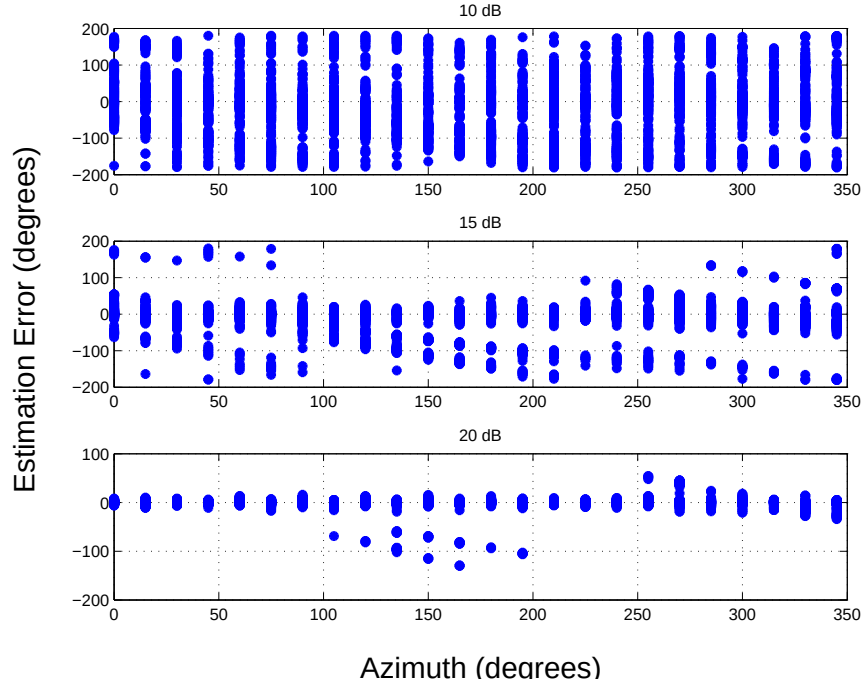
Figure B.10: f_c = 11 MHz Error Distribution vs. Azimuth for multiple SNR values using N_A = 16 feed points to synthesize a cube antenna pattern.
