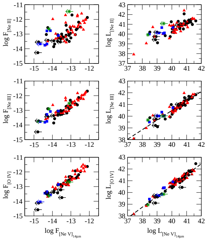
Figure 5. Correlation between [Ne II], [Ne III], [Ne V] 14 \mu\text{m} , and [O IV] fluxes and luminosities. Symbols are the same as in Figure 3. The dashed line represents the linear regression for the full sample (see Table 4). The statistical analysis and linear regression fits for these correlation are presented in Tables 2 and 4, respectively.
