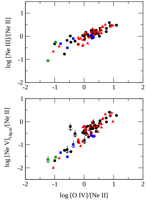
Figure 6. [Ne III]/[Ne II] and [Ne v] 14 \mu\text{m} /[Ne II] vs. [O IV]/[Ne II] ratios for Seyfert 1, Seyfert 2, BAT-detected AGNs, and LINERs in the BAT sample. Symbols are the same as in Figure 3. The \sim 62\% and \sim 72\% of the objects in our sample have [Ne III]/[Ne II] and [O IV]/[Ne II] have ratios bigger than unity, which has been shown to be typical of AGN-ionized emission-line gas (e.g., Meléndez et al. 2008a). The [Ne v] and [O IV] ratios appear well correlated, as expected given the tight correlation seen in Figure 5.
