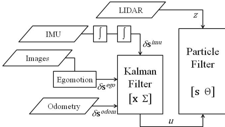
Figure 10. System diagram of the novel SLAM solution. A Kalman filter takes twice-integrated IMU measurements, egomotion from stereo images, and vehicle odometry as input. It then provides u to a particle filter that also takes LIDAR ranges z .
