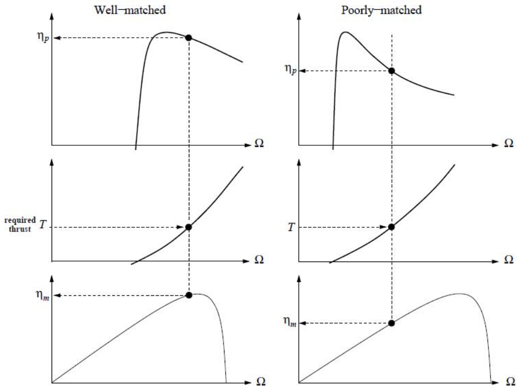
Figure 19: Well-Matched and Poorly-Matched Motor and Propeller Pairs
