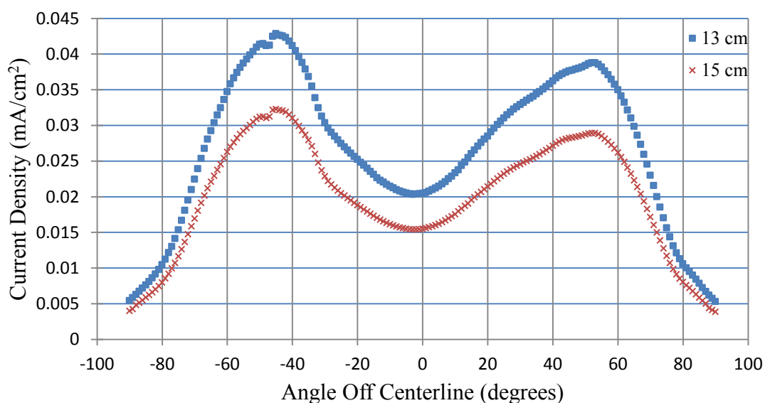
Figure 43. Current density curves for 4.7 W operating condition with thruster rotated 90 degrees with respect to configuration for Figure 40.
