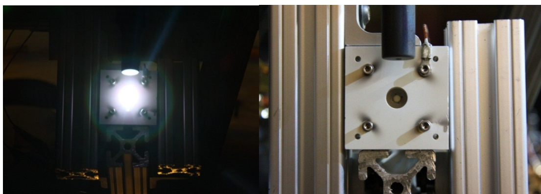
a) Thruster operating at peak of 25 W b) No damage to BN anode post.
