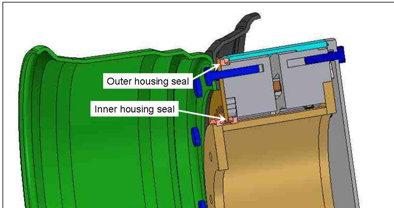
Figure 1 - Sealing
