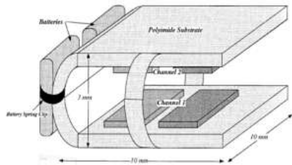
Figure 15: Graphical representation of a EMG backpack designed for M.sexta
