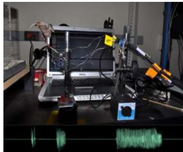
Figure 26: EMG signals from a M.sexta , using fine wire implants; the recorded signals are superimposed below the picture
