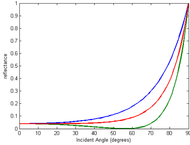
Figure 2. Reflectance calculated with Fresnel equations for the air to skin interface, showing S polarized (blue), P polarized (green), and unpolarized light (red) dependent on incident angle.
