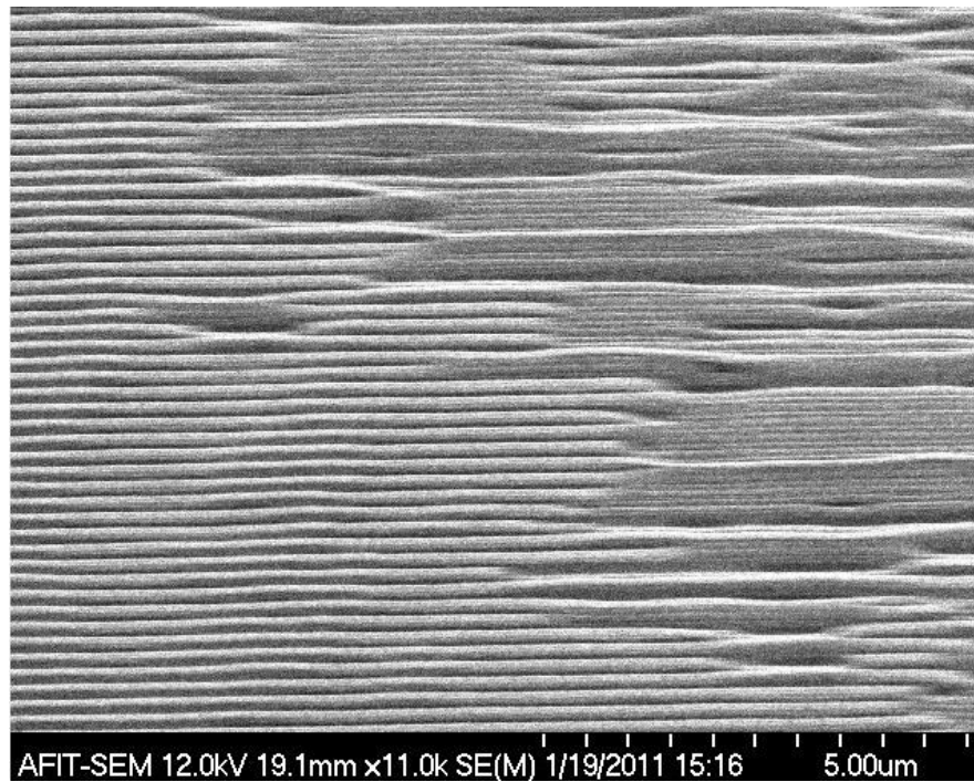
Fig 4.6 Side-view of 230-nm S1805 features.
