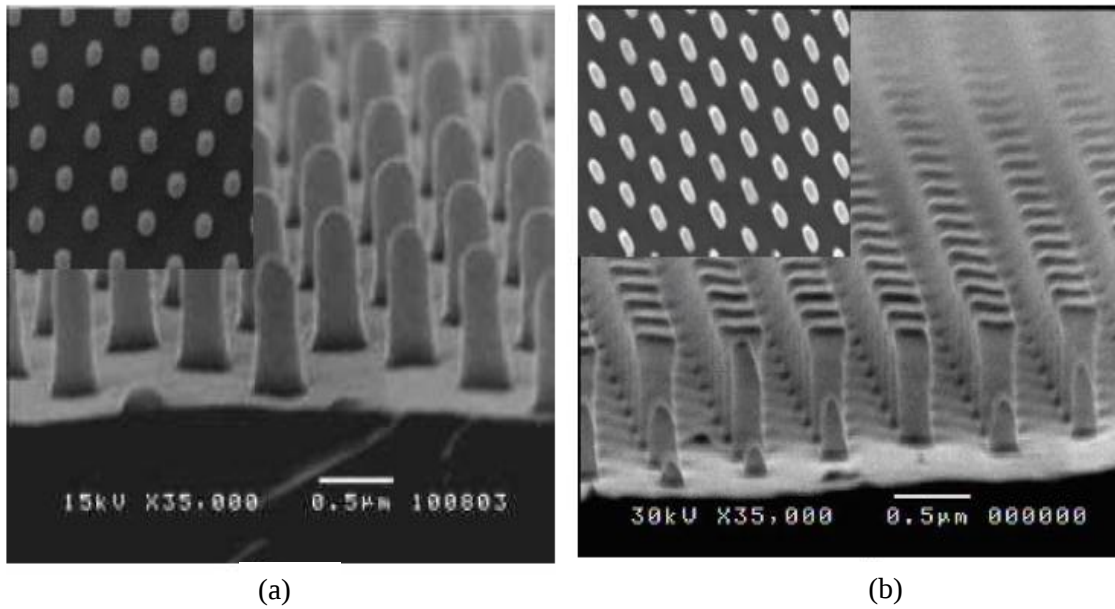
Fig. 2.14 2D structures recorded by double holographic exposure. (a) Cubic lattice and (b) hexagonal lattice. The size of the scale bar is 0.5μm [17].
