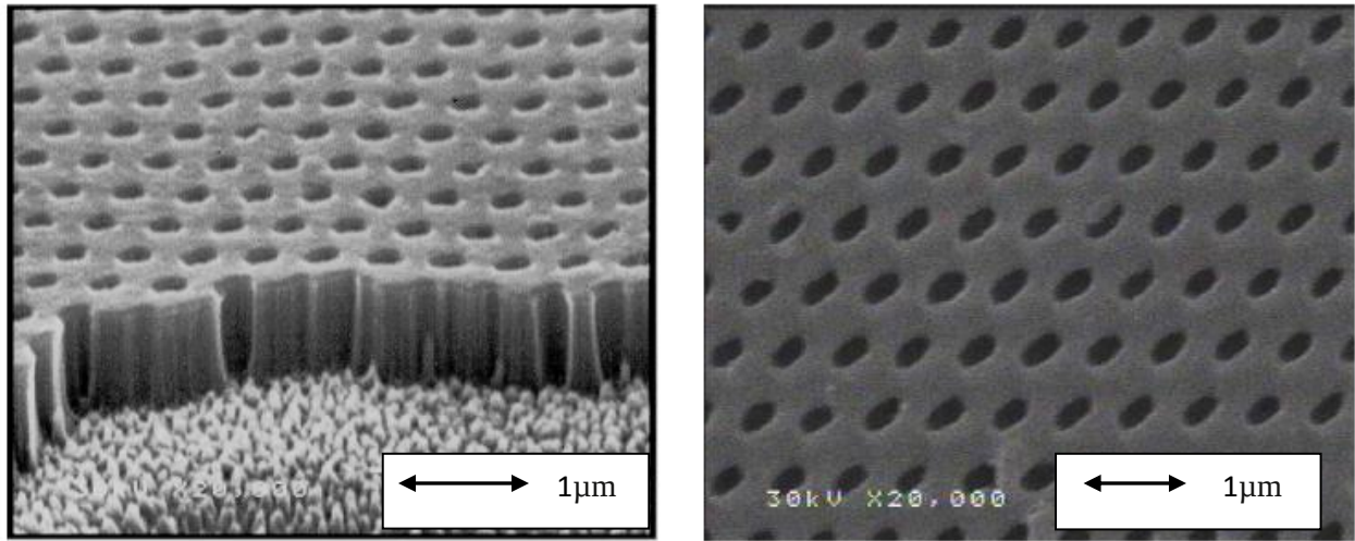
Fig. 2.16 2D structures with hexagonal lattice recorded in a-C:H film. The size of the scale bar is 1μm [17].
