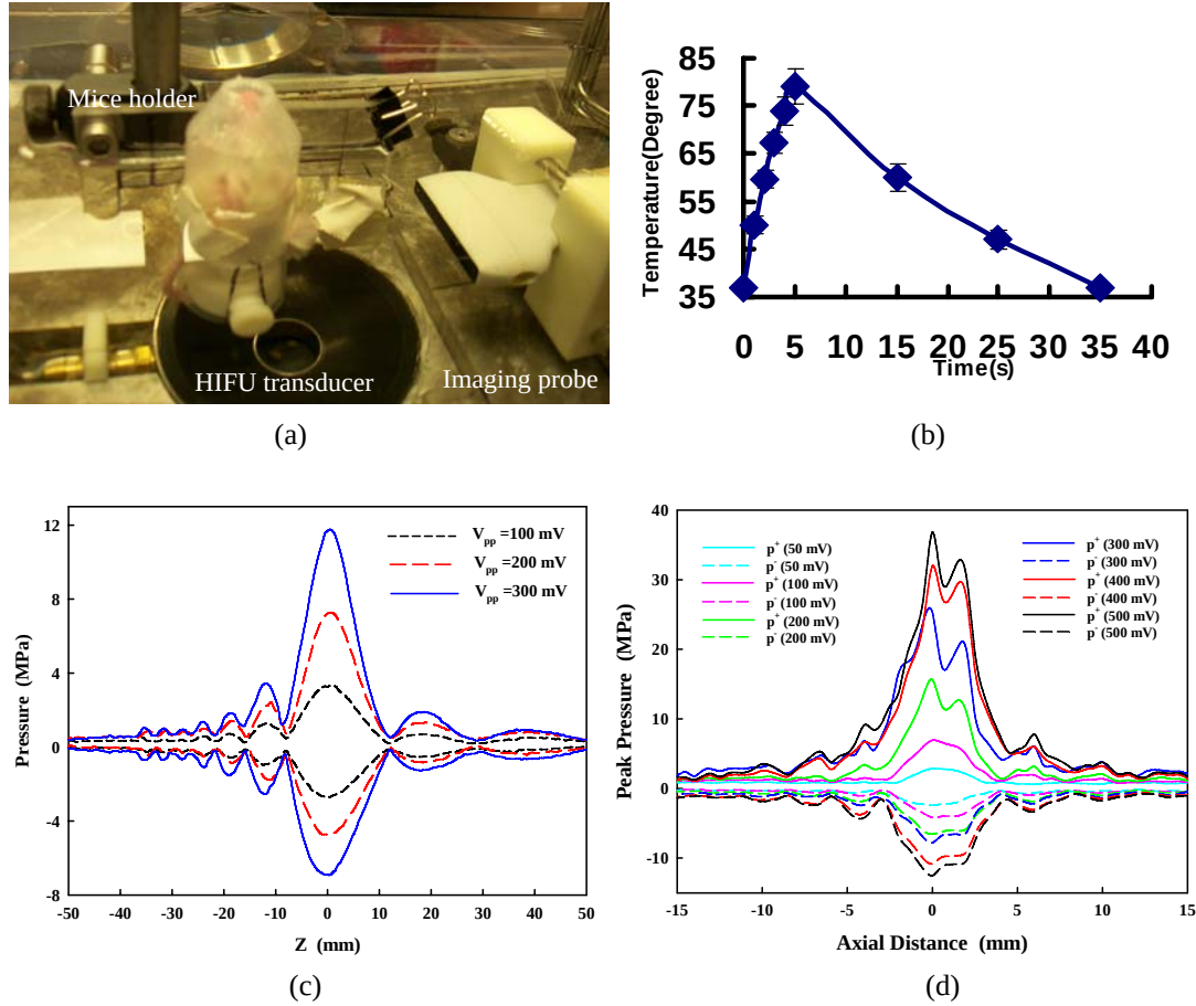
Fig. 1 (a) Experimental HIFU system (b) Representative temperature profile at HIFU focus (c)-(d) Axial pressure distribution at 1.1MHz and 3.3MHz
